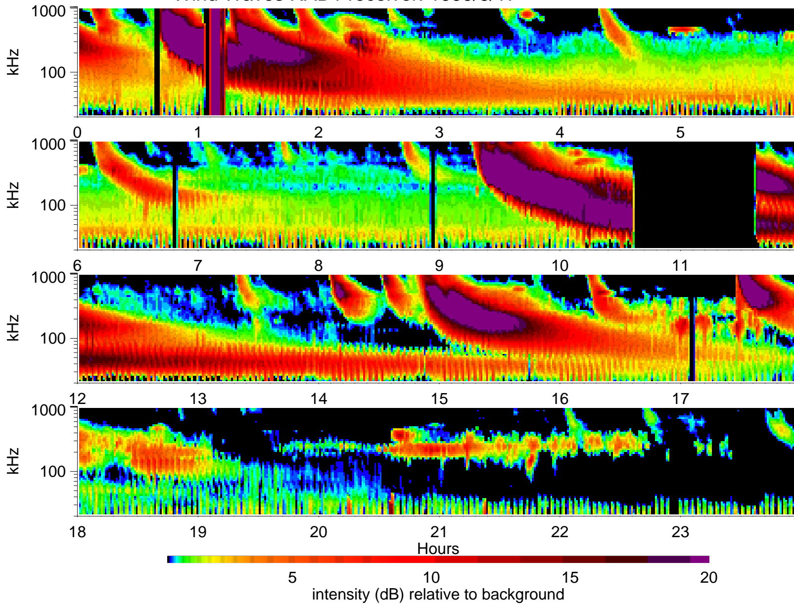
Wind Waves RAD1 receiver: 1999/6/17
