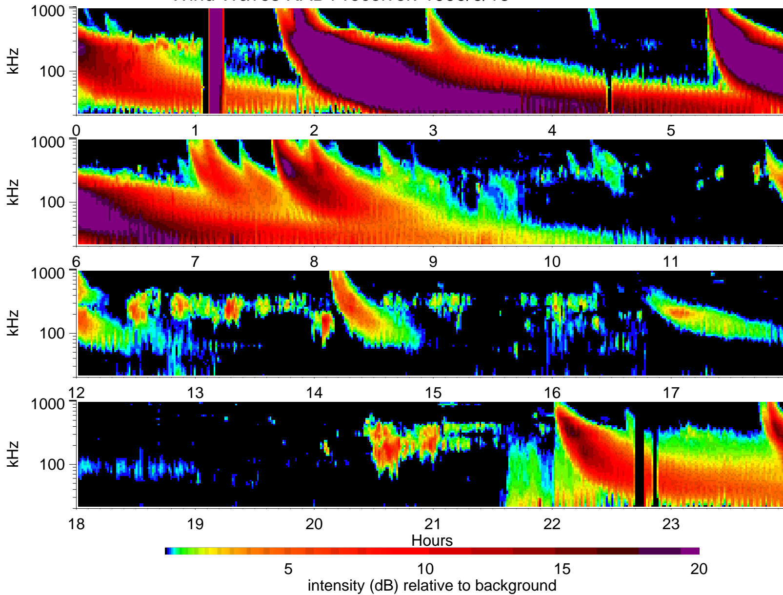
Wind Waves RAD1 receiver: 1999/6/13
