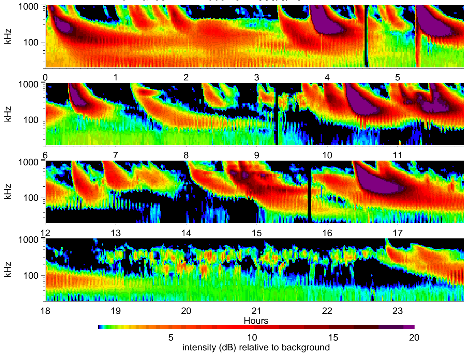
Wind Waves RAD1 receiver: 1999/6/10
