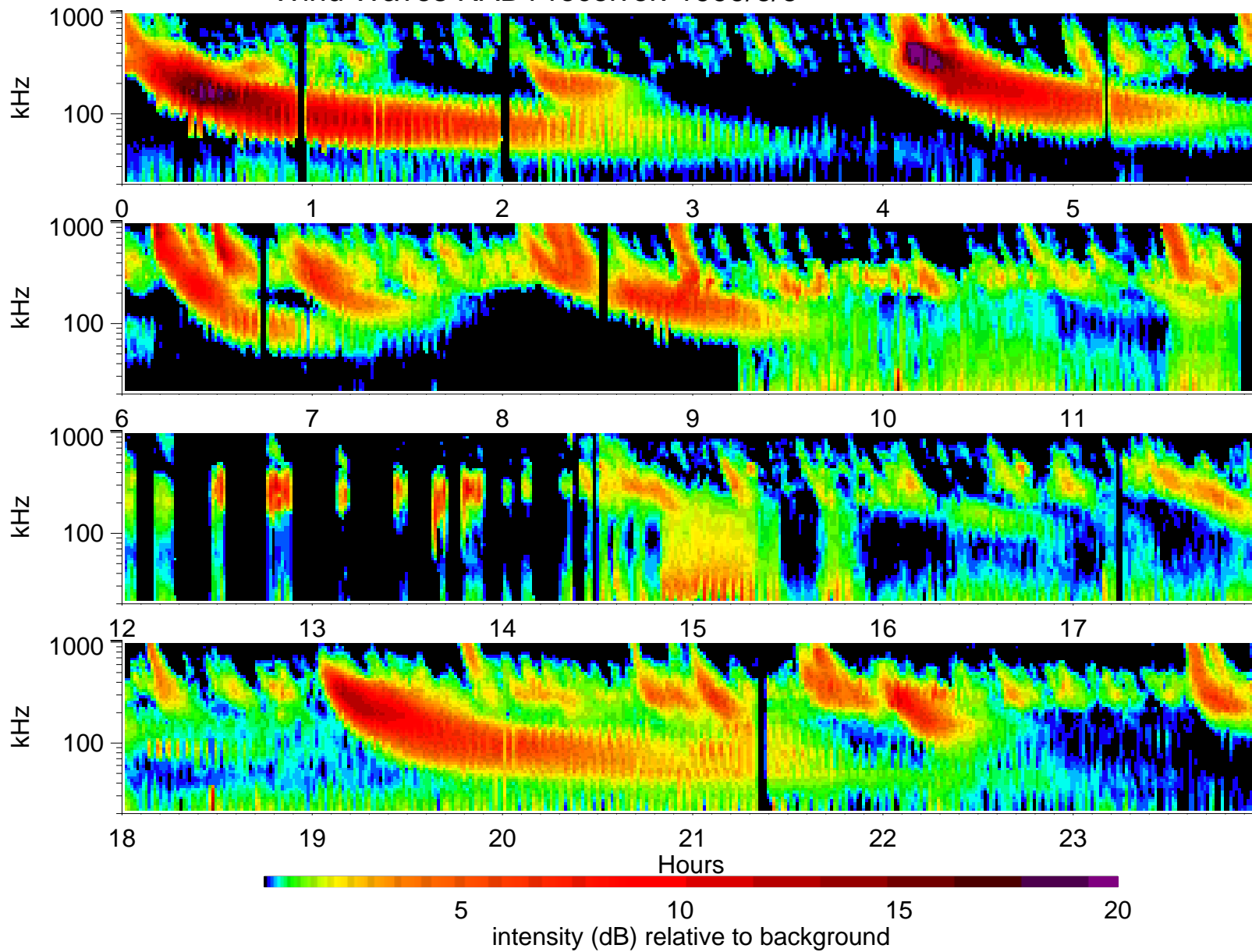
Wind Waves RAD1 receiver: 1999/6/6
