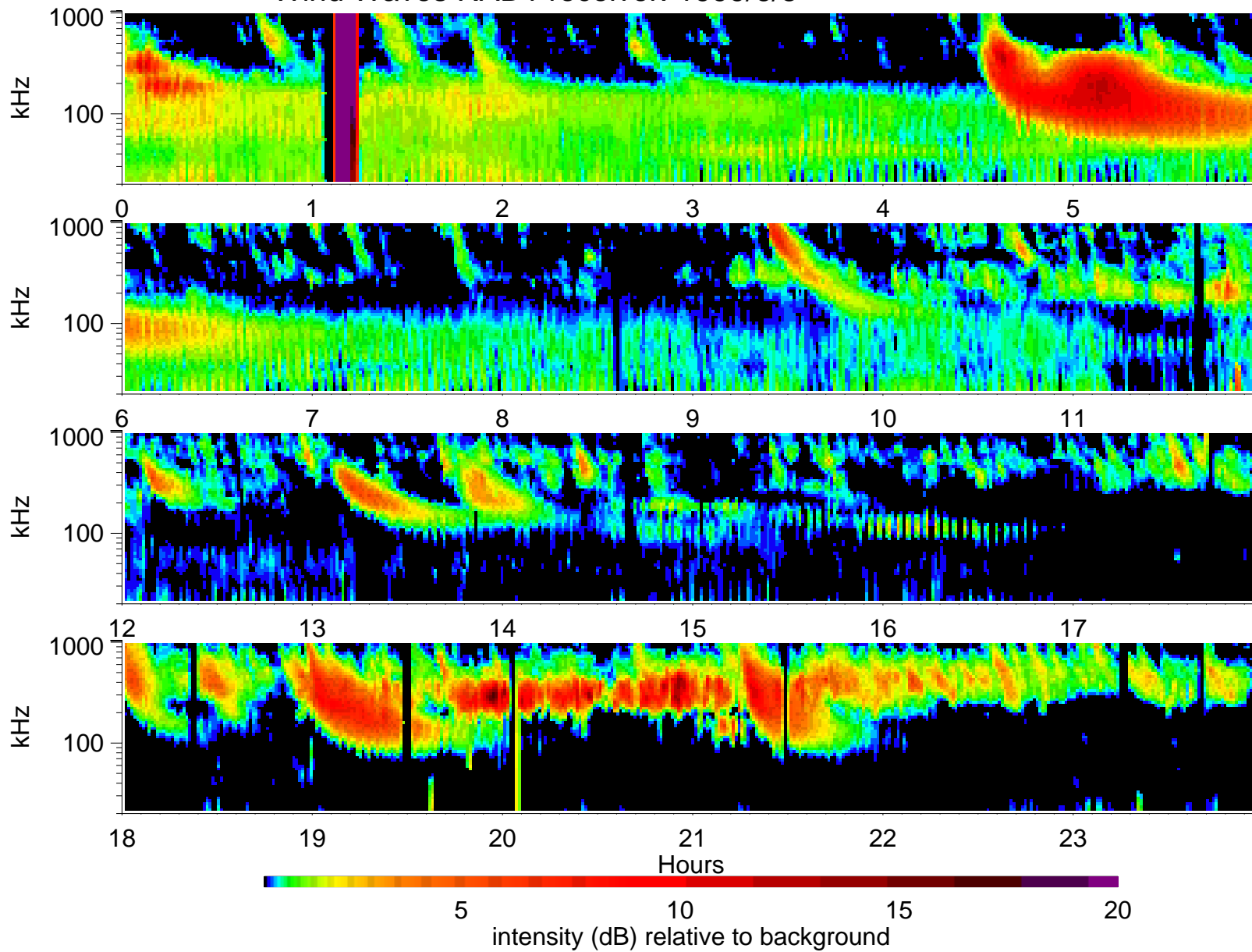
Wind Waves RAD1 receiver: 1999/6/5
