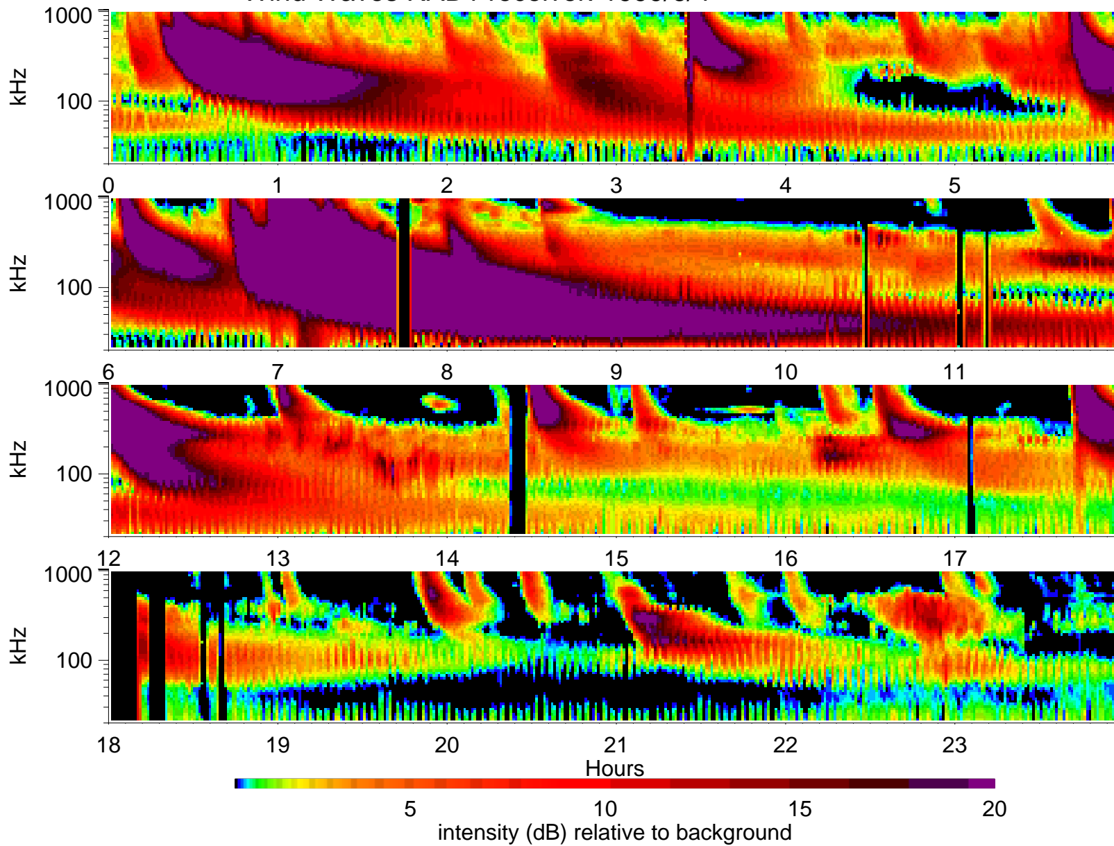
Wind Waves RAD1 receiver: 1999/6/4
