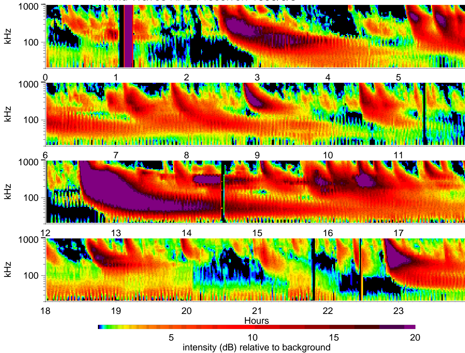
Wind Waves RAD1 receiver: 1999/6/3
