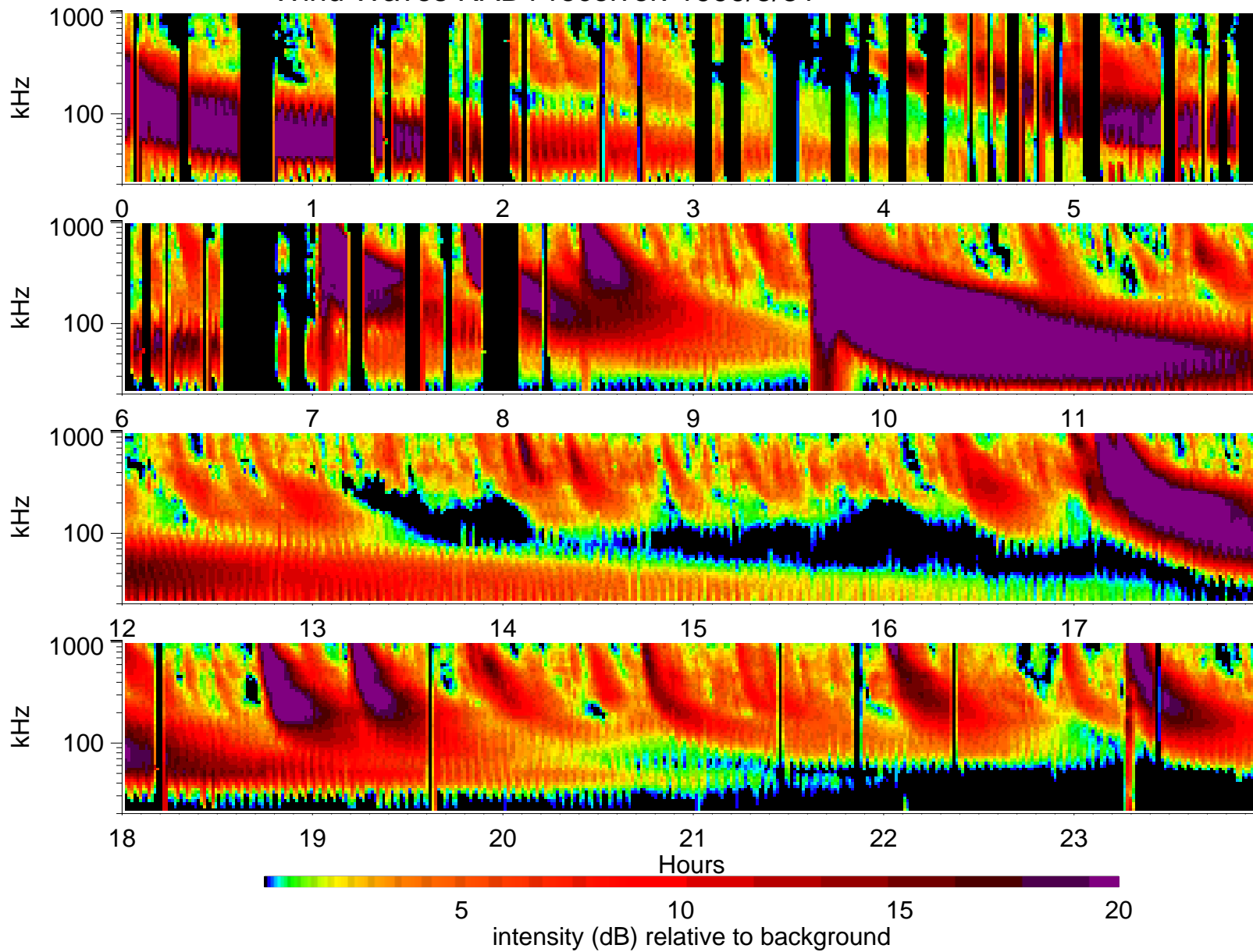
Wind Waves RAD1 receiver: 1999/5/31
