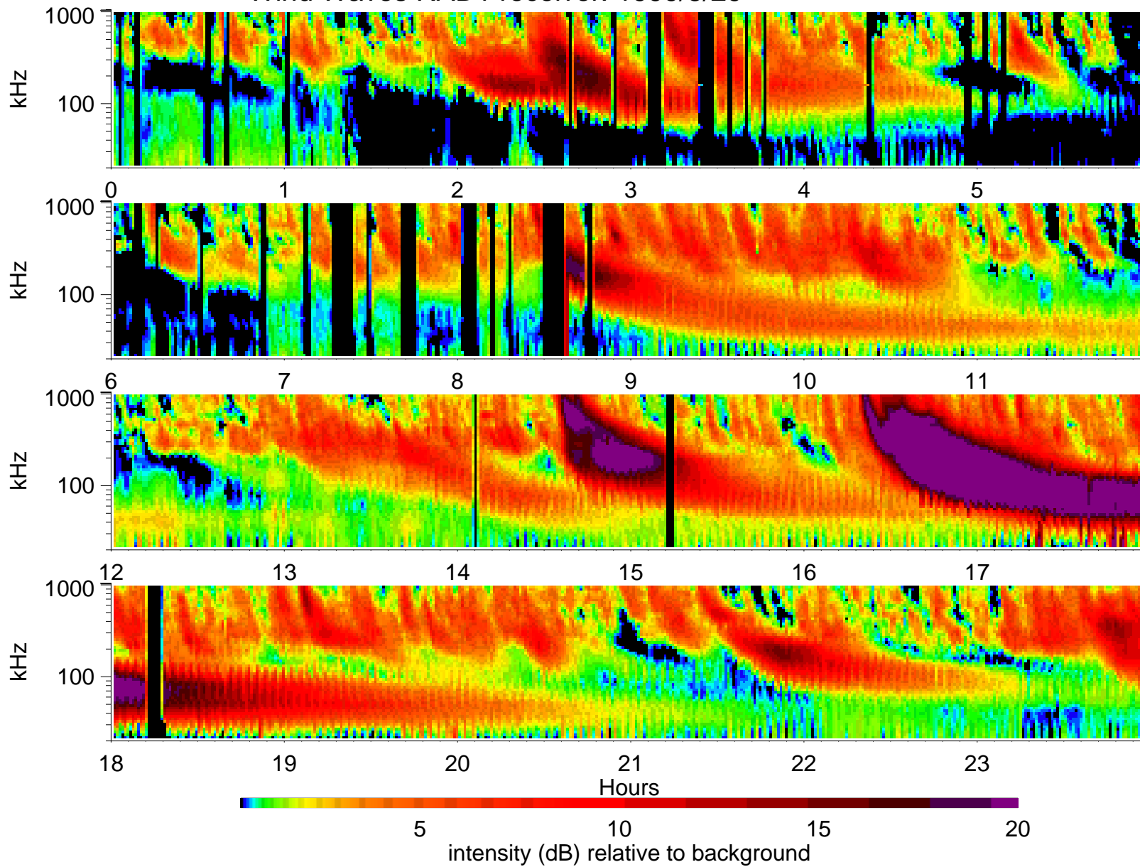
Wind Waves RAD1 receiver: 1999/5/29
