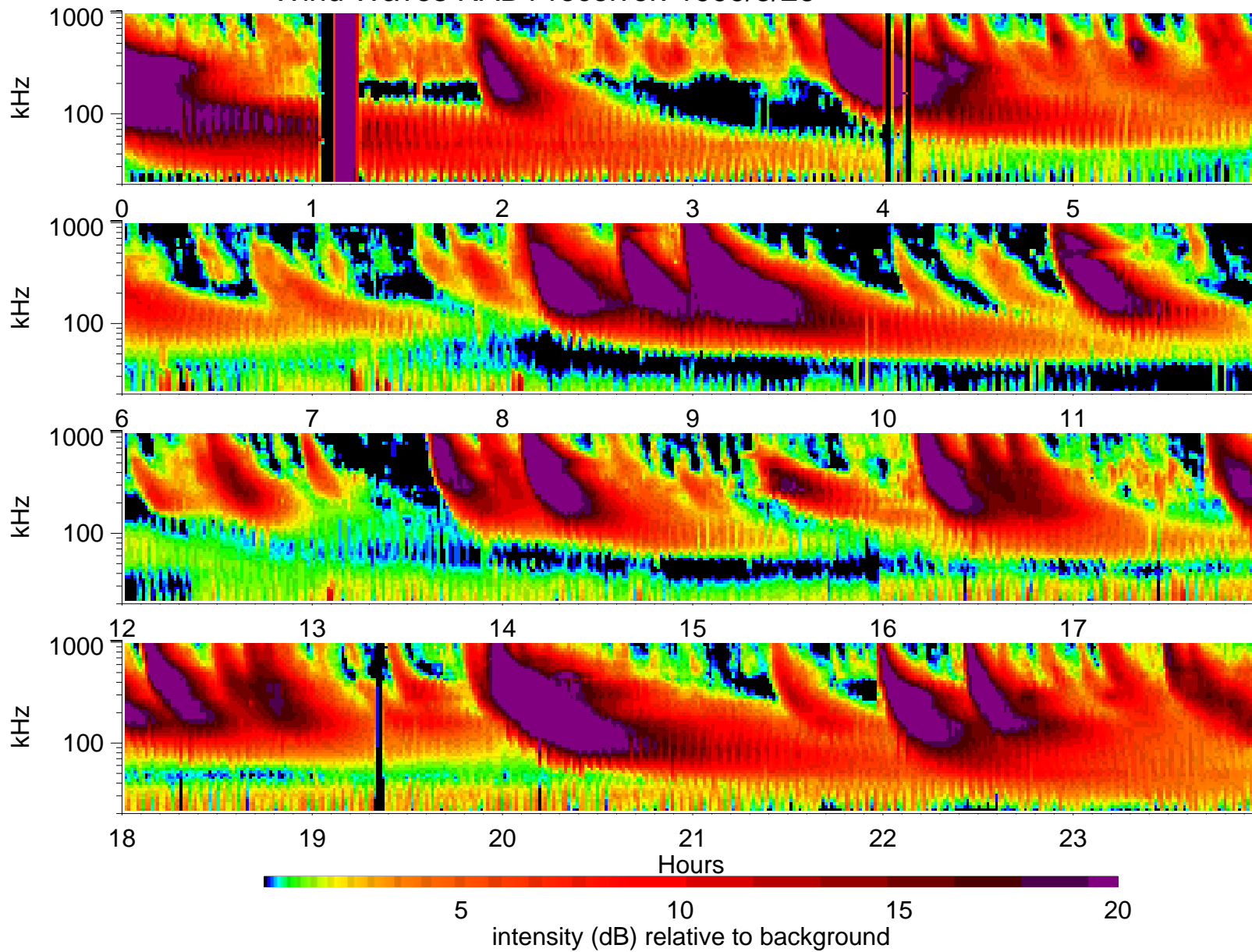
Wind Waves RAD1 receiver: 1999/5/26
