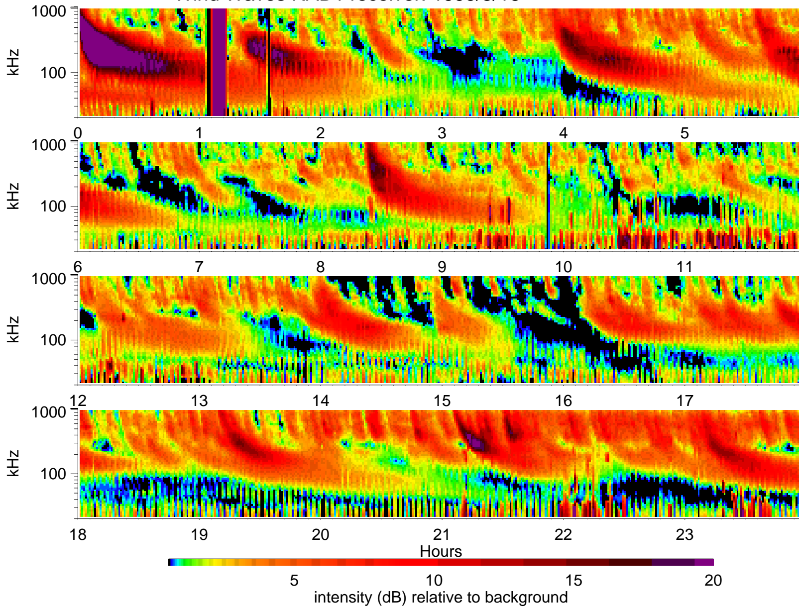
Wind Waves RAD1 receiver: 1999/5/16
