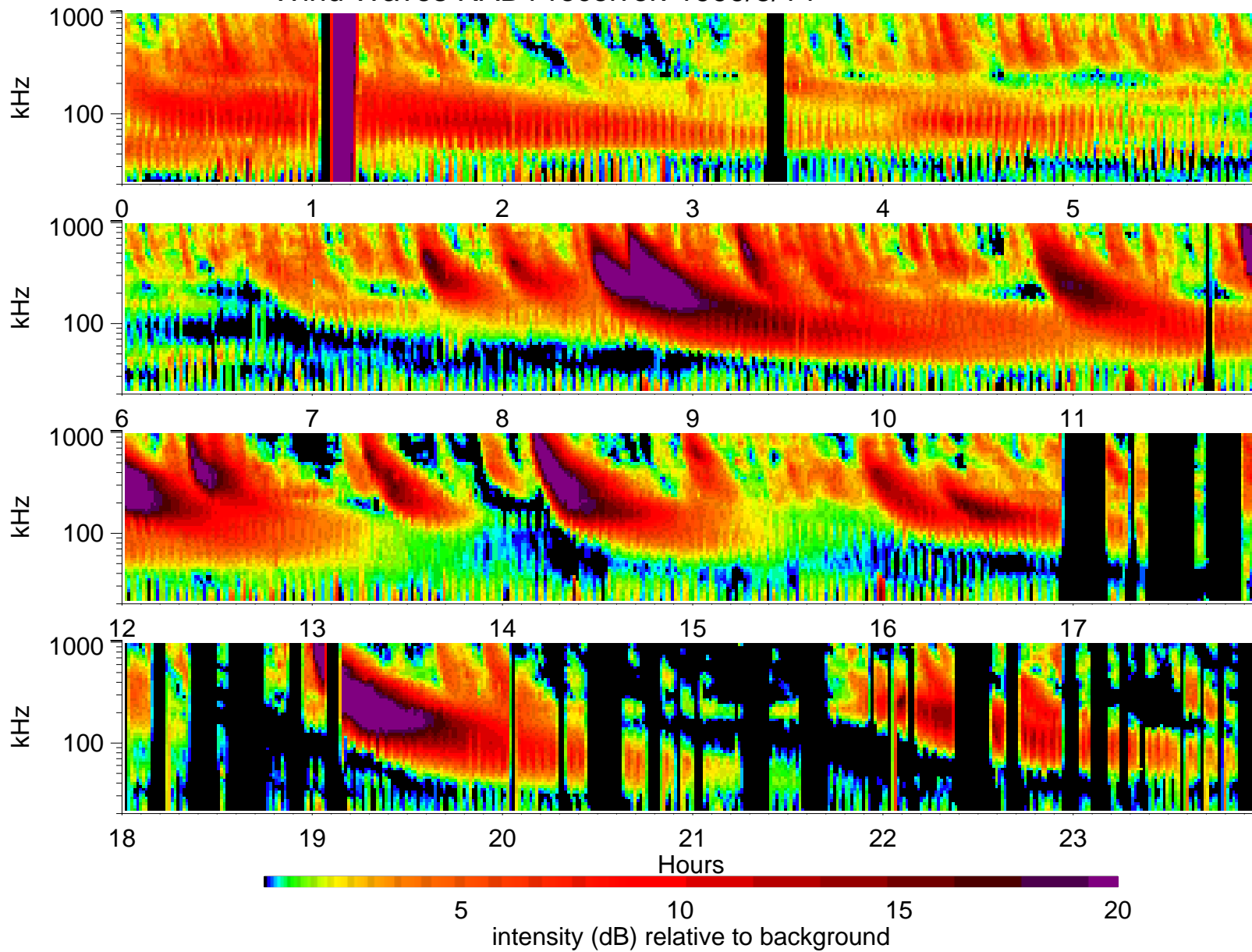
Wind Waves RAD1 receiver: 1999/5/14
