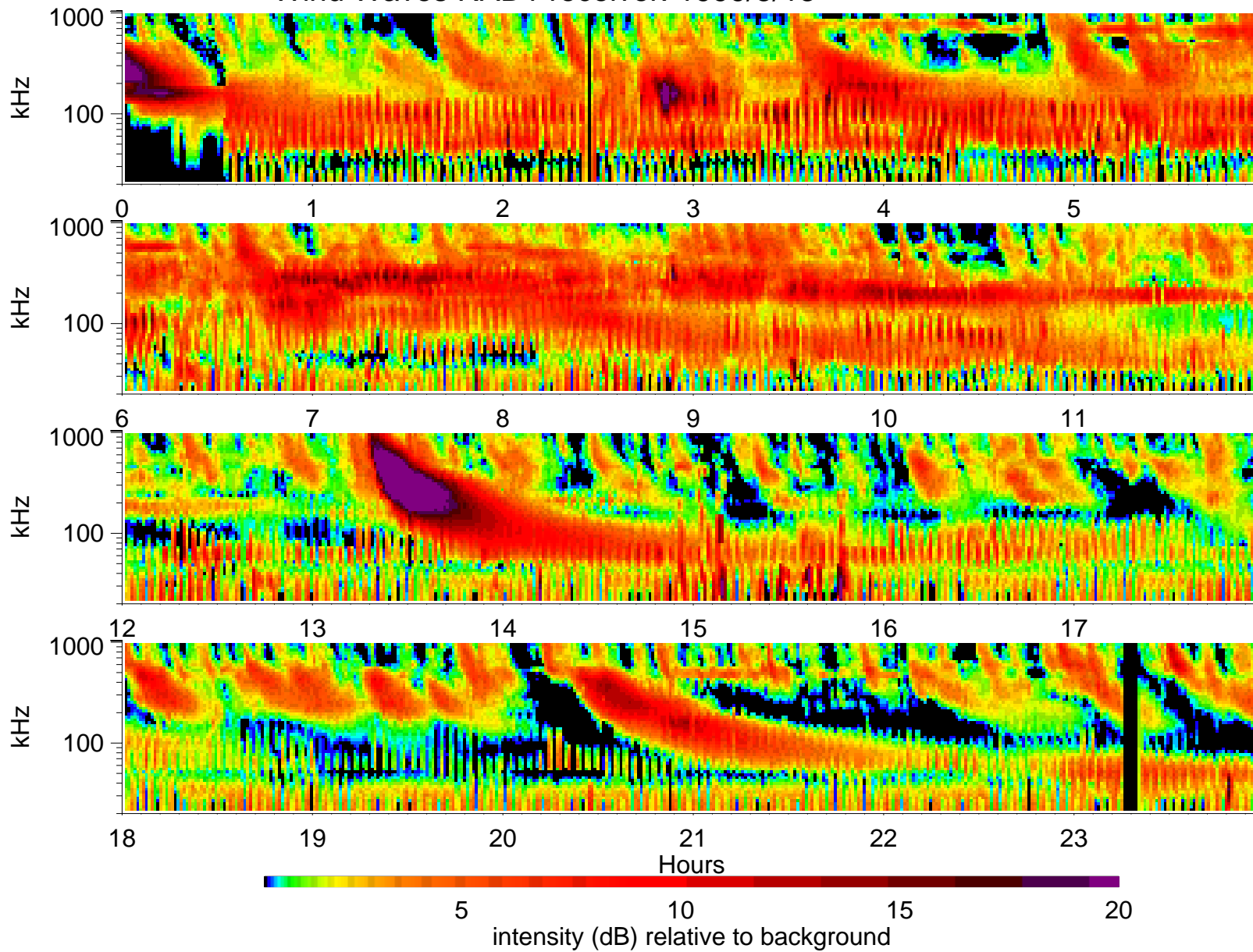
Wind Waves RAD1 receiver: 1999/5/13
