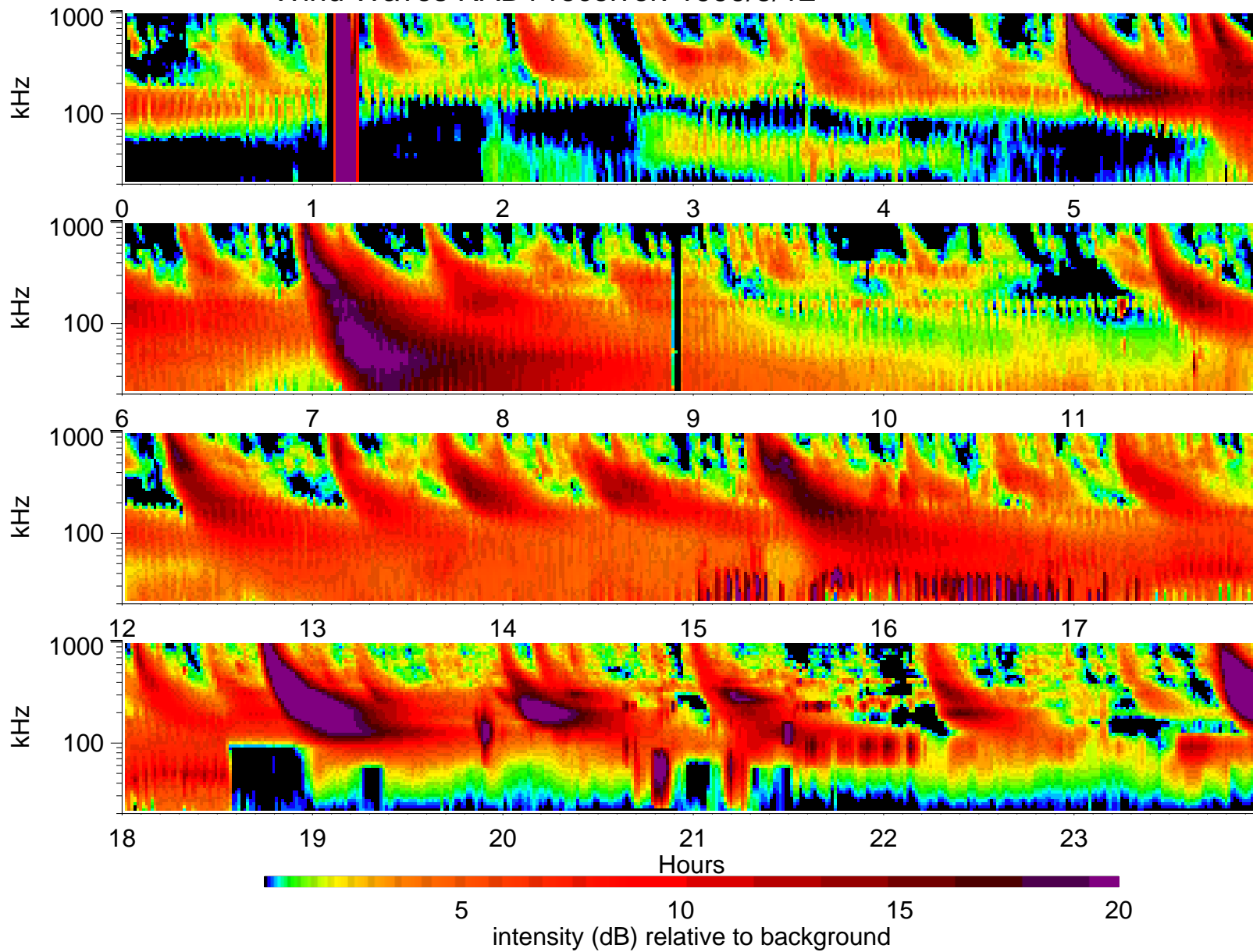
Wind Waves RAD1 receiver: 1999/5/12
