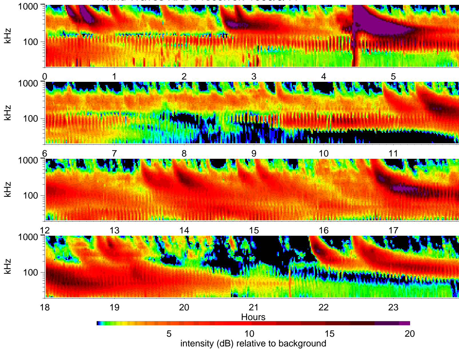
Wind Waves RAD1 receiver: 1999/5/11
