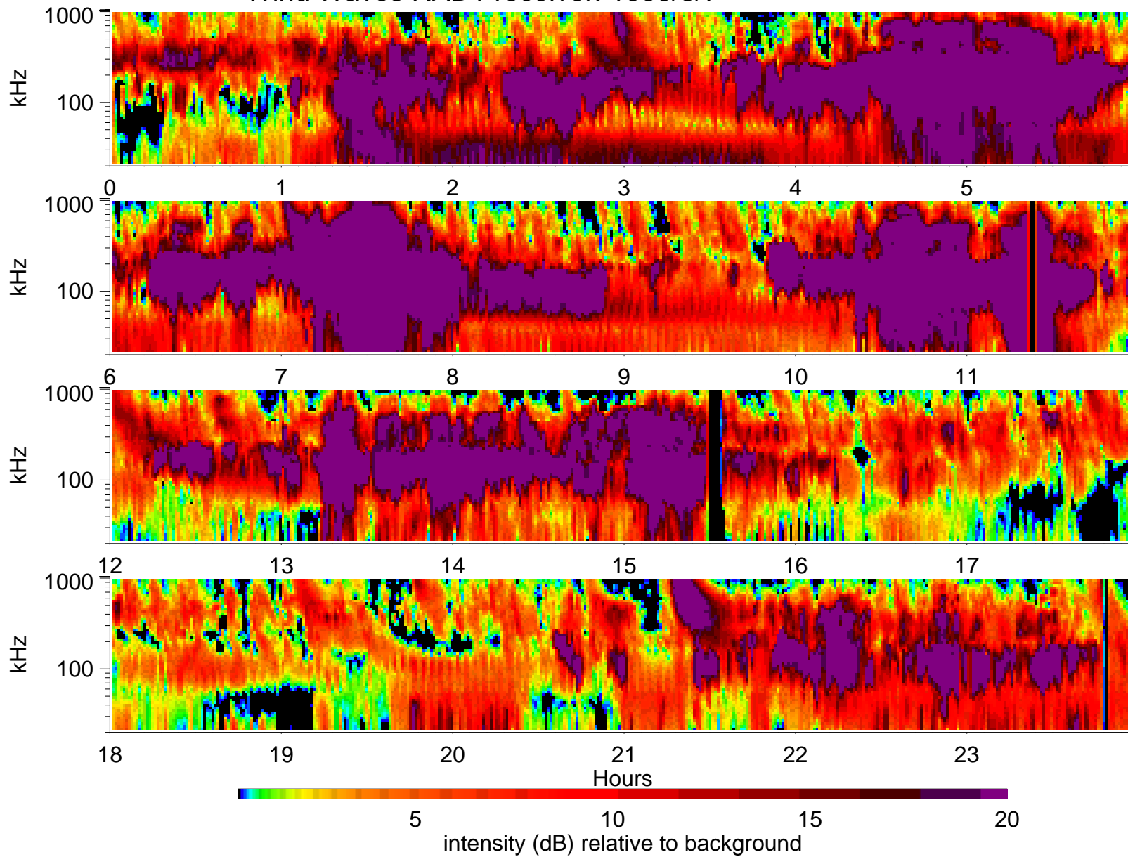
Wind Waves RAD1 receiver: 1999/5/7
