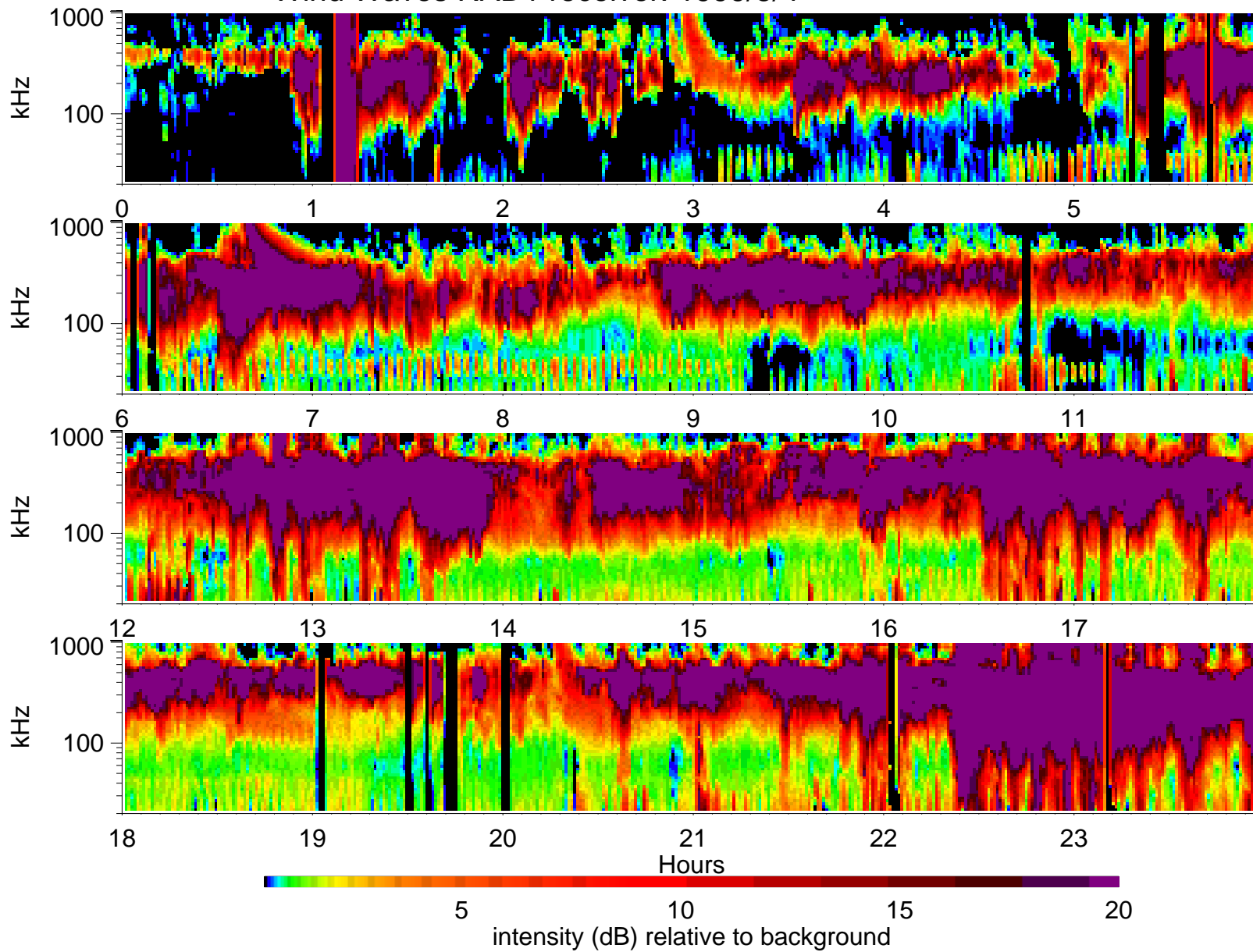
Wind Waves RAD1 receiver: 1999/5/4
