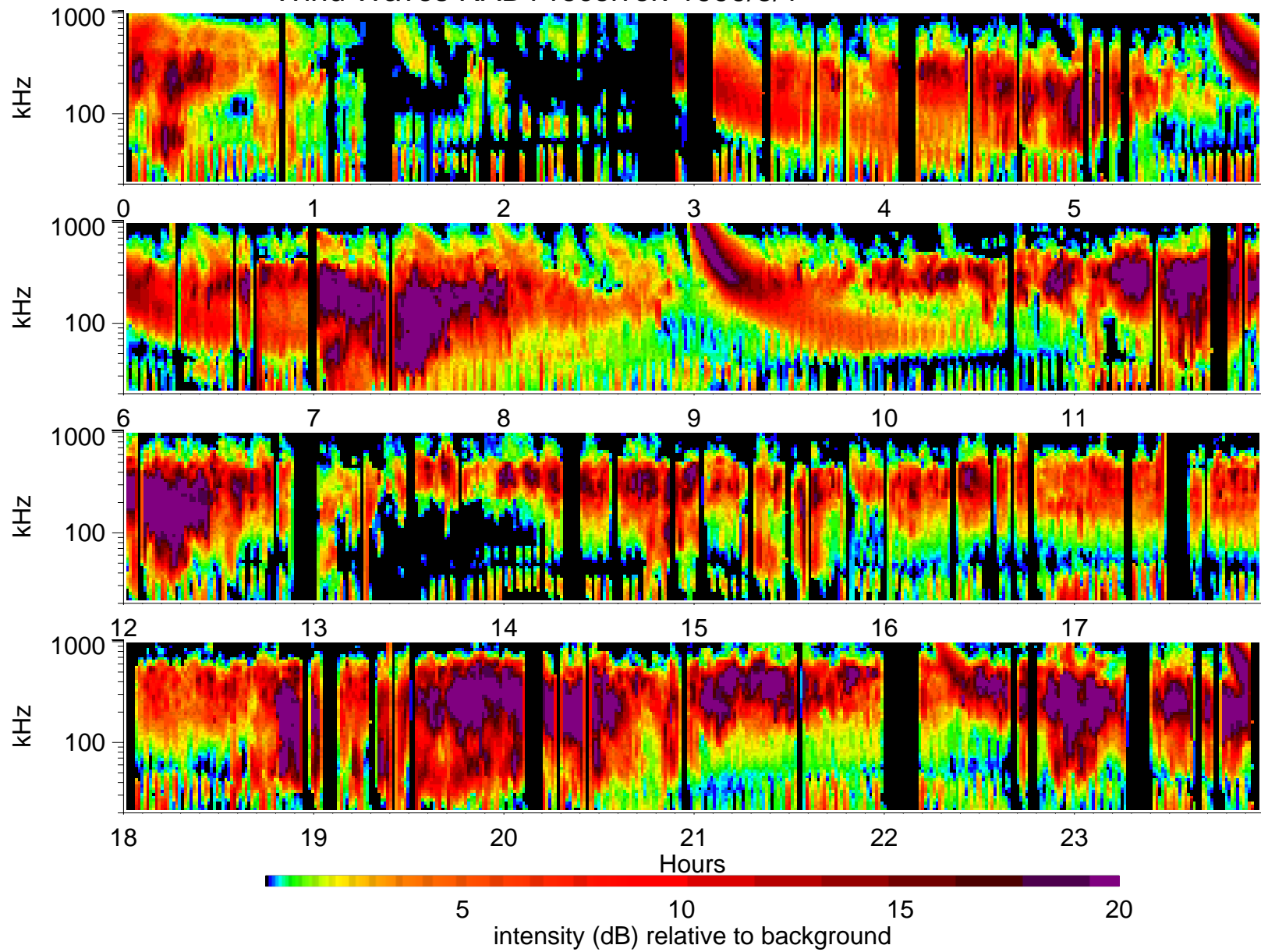
Wind Waves RAD1 receiver: 1999/5/1
