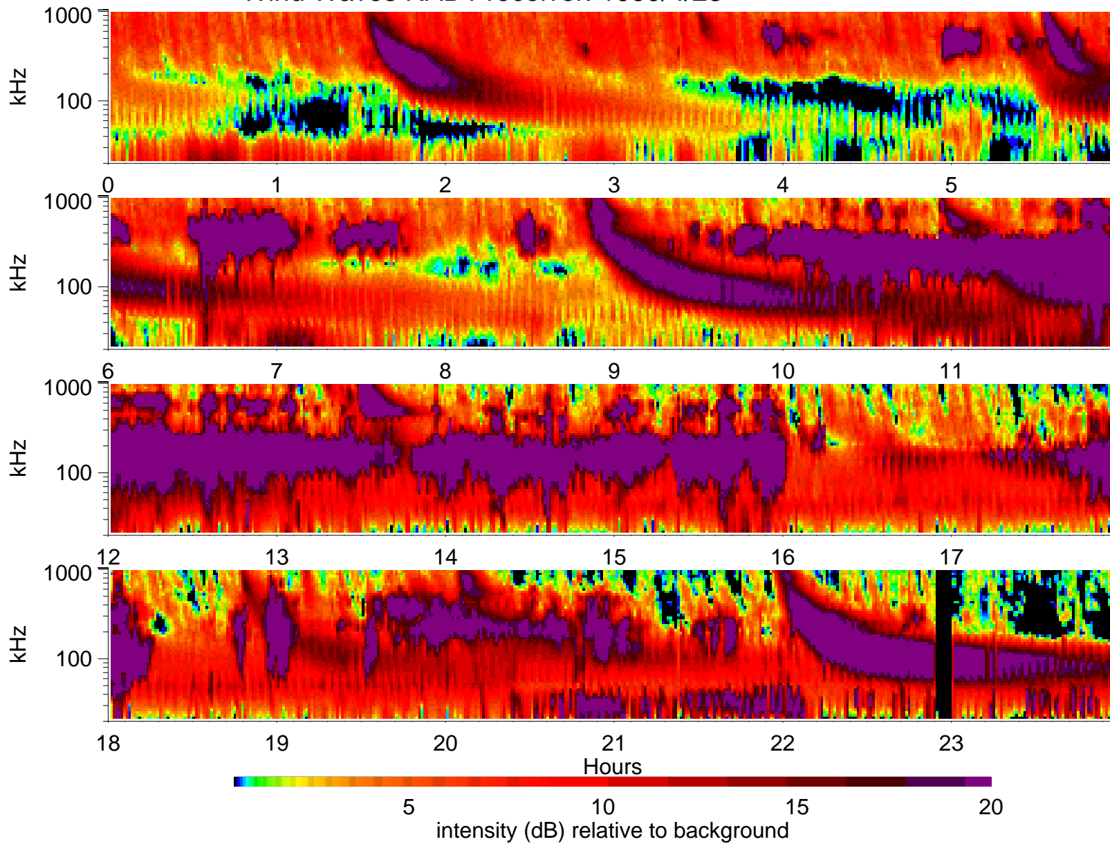
Wind Waves RAD1 receiver: 1999/4/23
