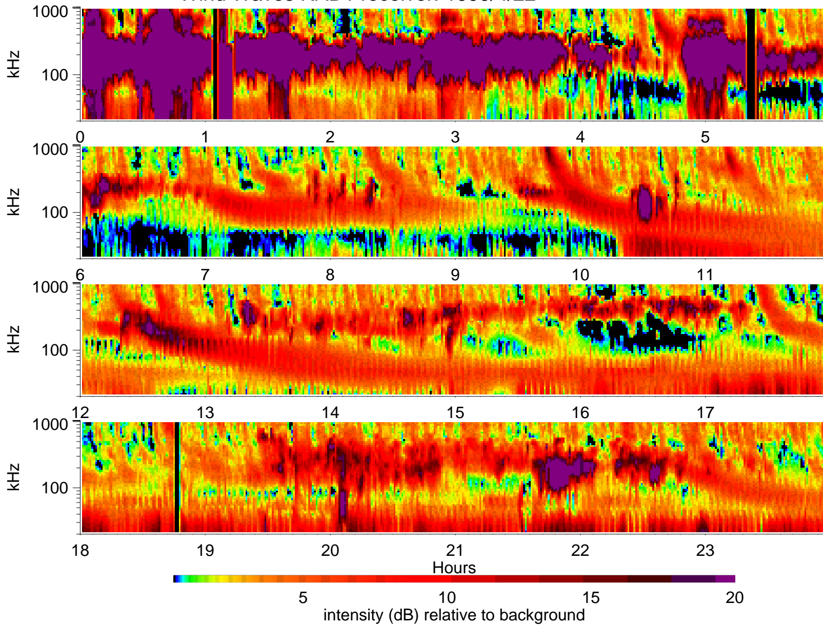
Wind Waves RAD1 receiver: 1999/4/22
