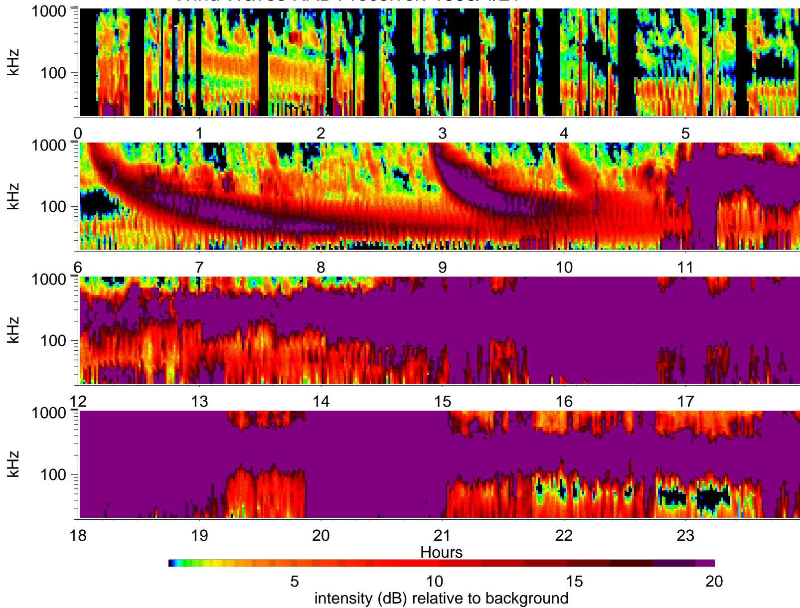
Wind Waves RAD1 receiver: 1999/4/21
