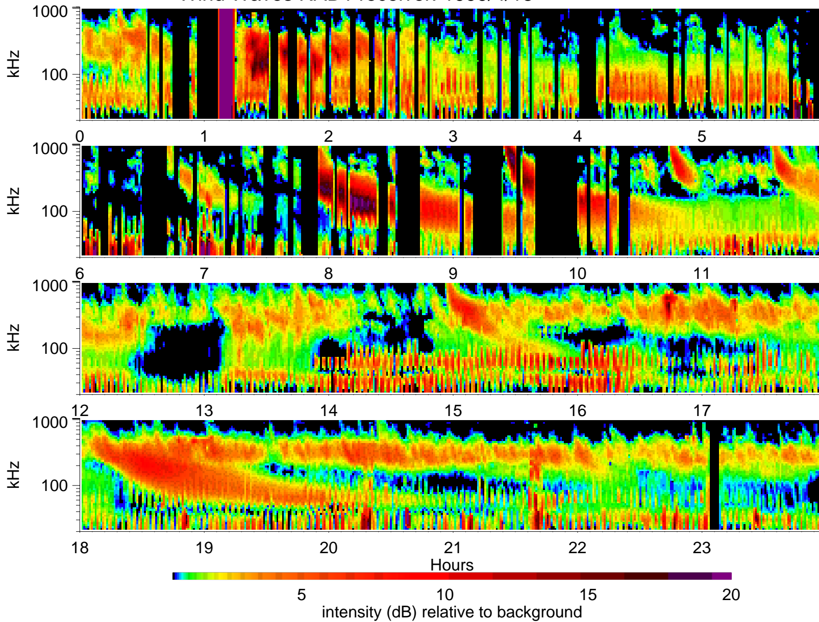
Wind Waves RAD1 receiver: 1999/4/18
