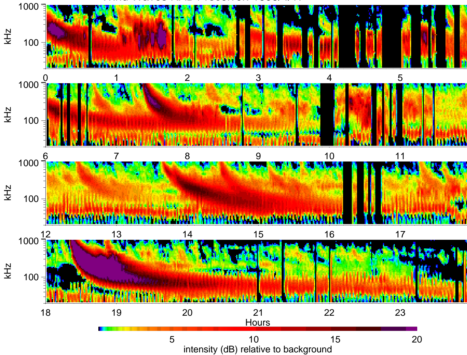
Wind Waves RAD1 receiver: 1999/4/17
