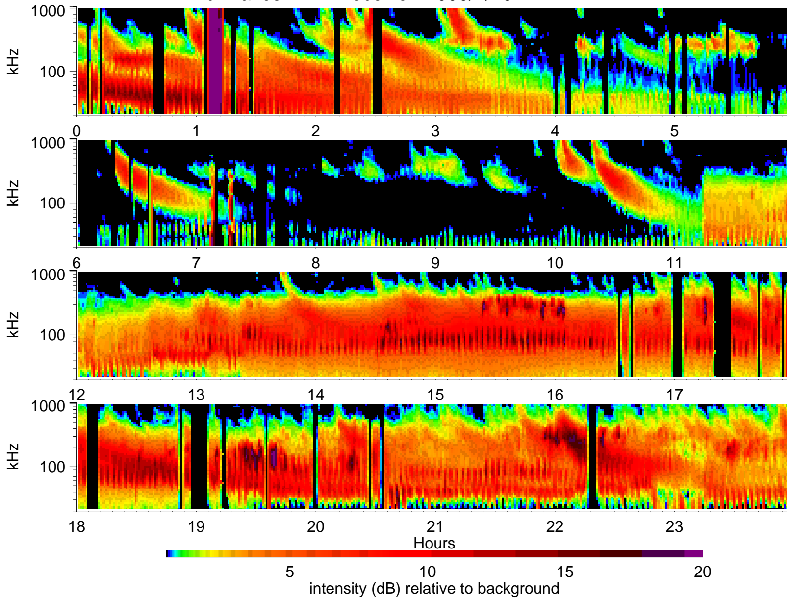
Wind Waves RAD1 receiver: 1999/4/16
