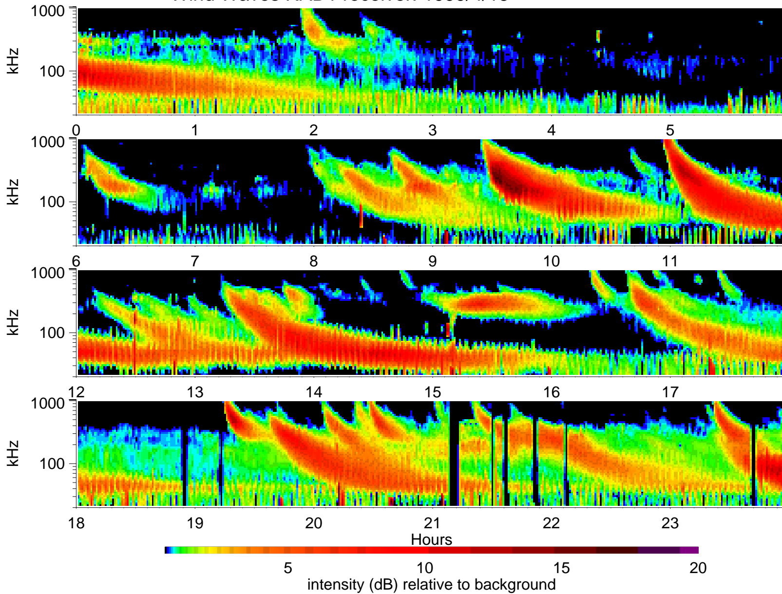
Wind Waves RAD1 receiver: 1999/4/15
