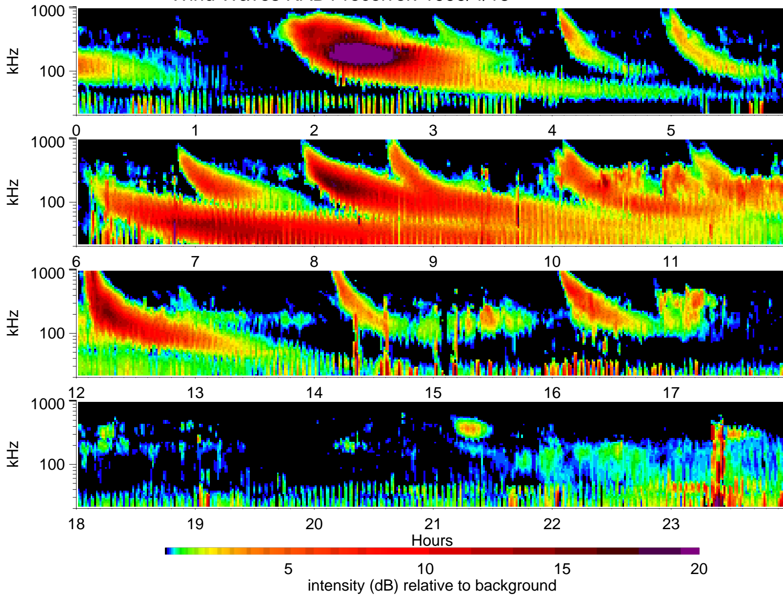
Wind Waves RAD1 receiver: 1999/4/13
