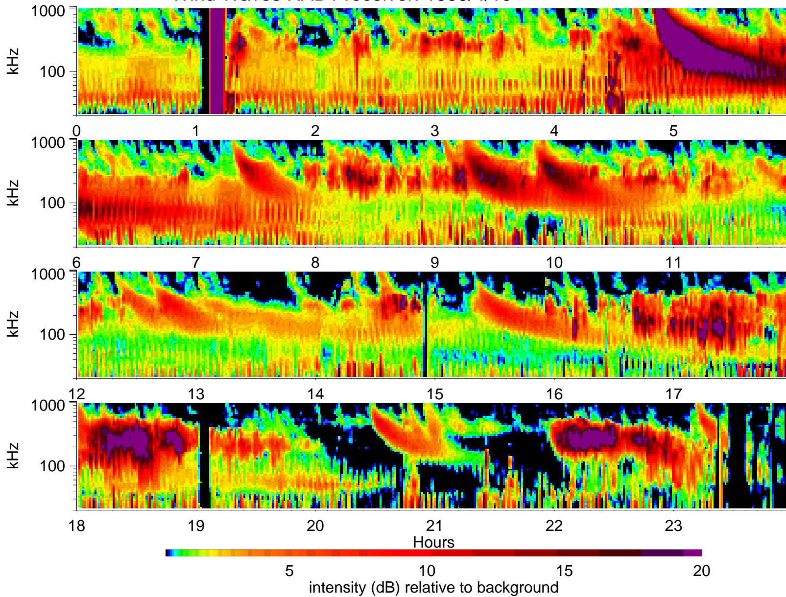
Wind Waves RAD1 receiver: 1999/4/10
