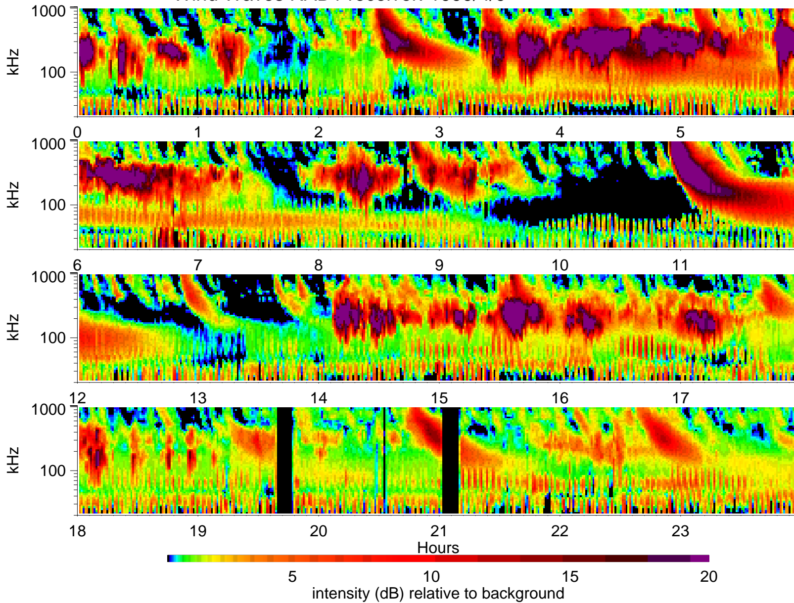
Wind Waves RAD1 receiver: 1999/4/9
