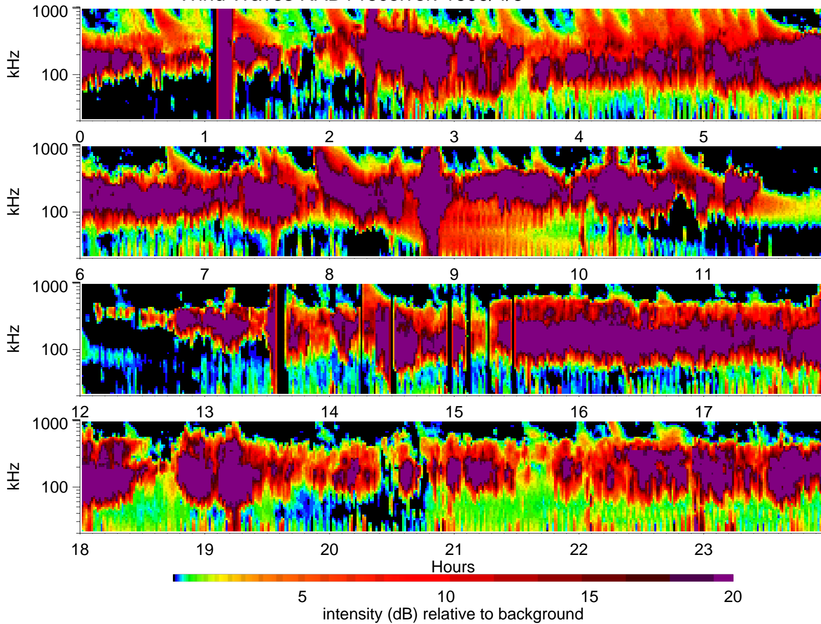
Wind Waves RAD1 receiver: 1999/4/6
