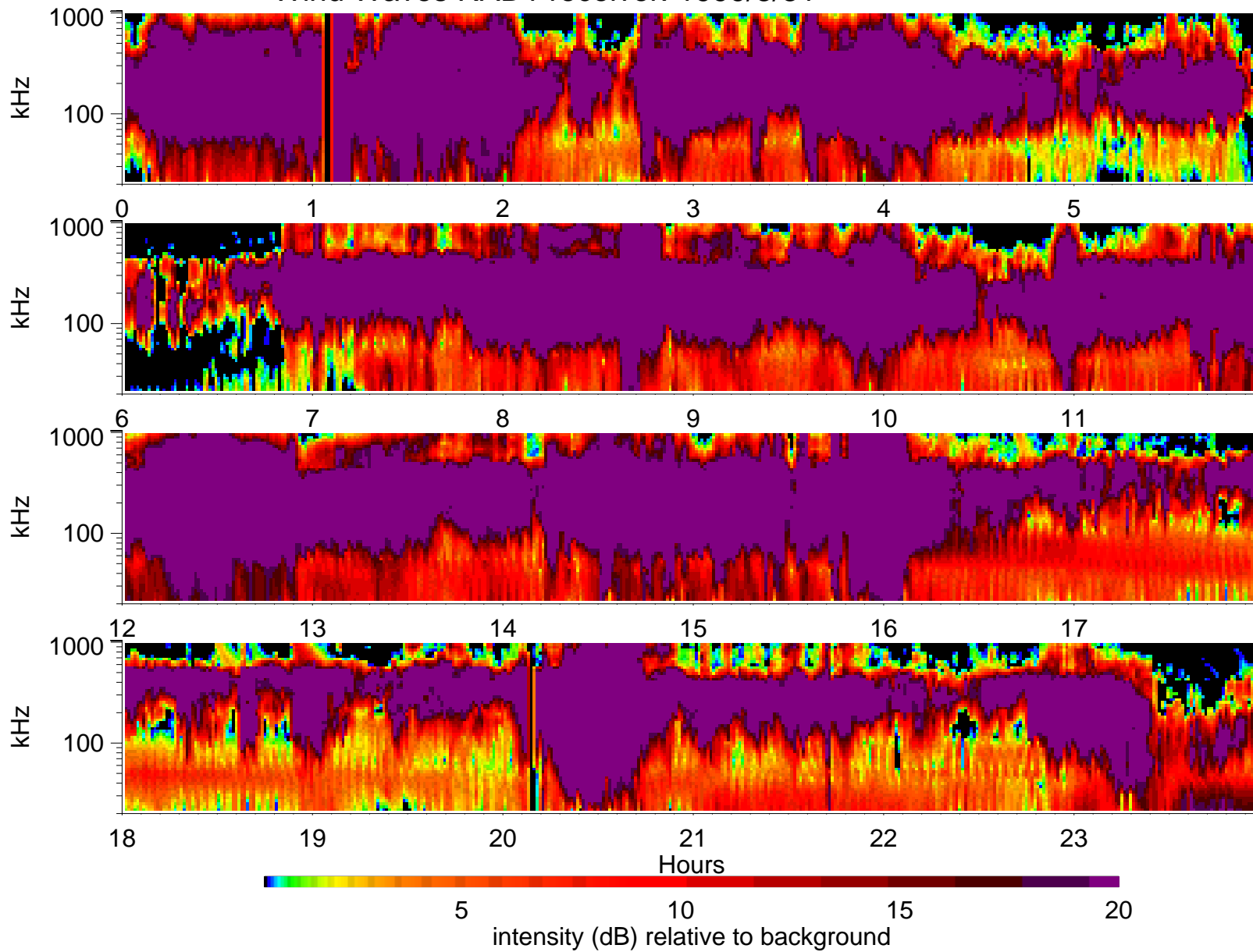
Wind Waves RAD1 receiver: 1999/3/31
