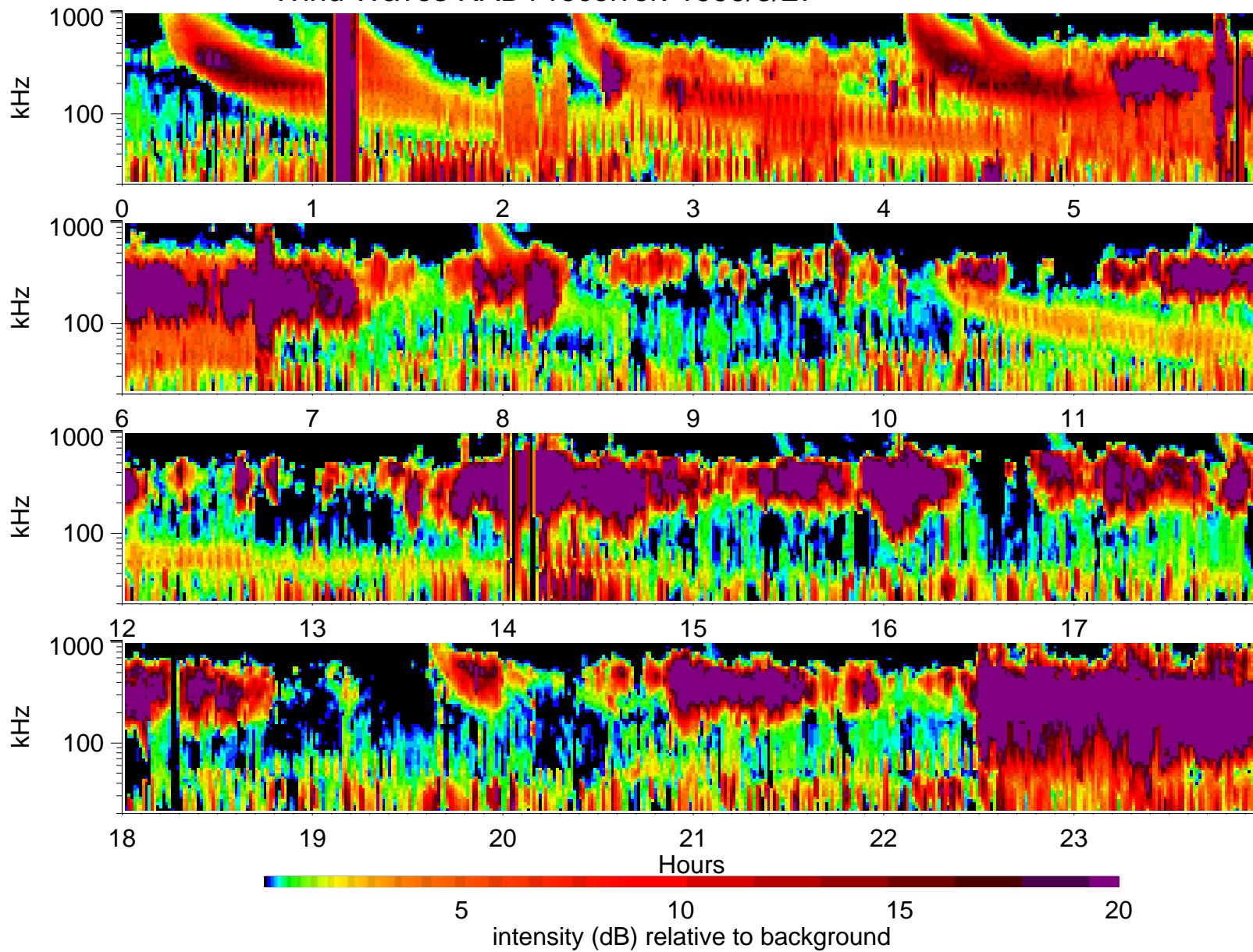
Wind Waves RAD1 receiver: 1999/3/27
