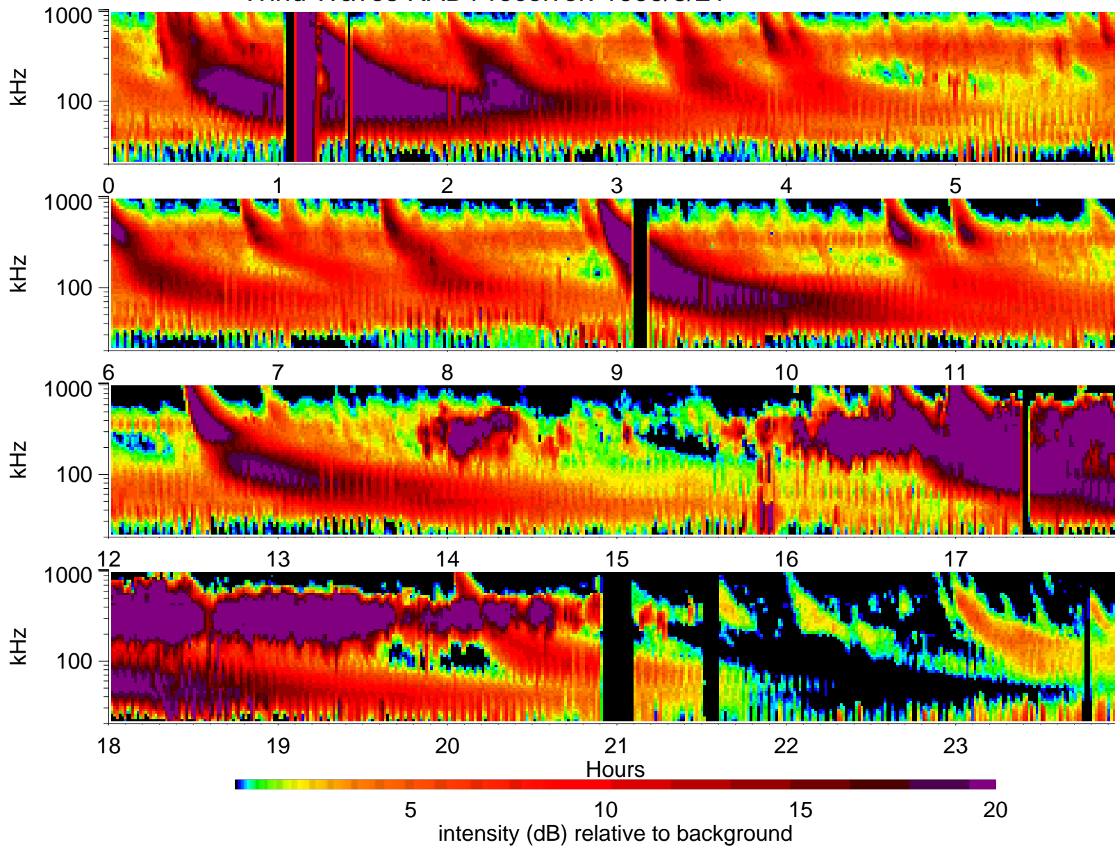
Wind Waves RAD1 receiver: 1999/3/21
