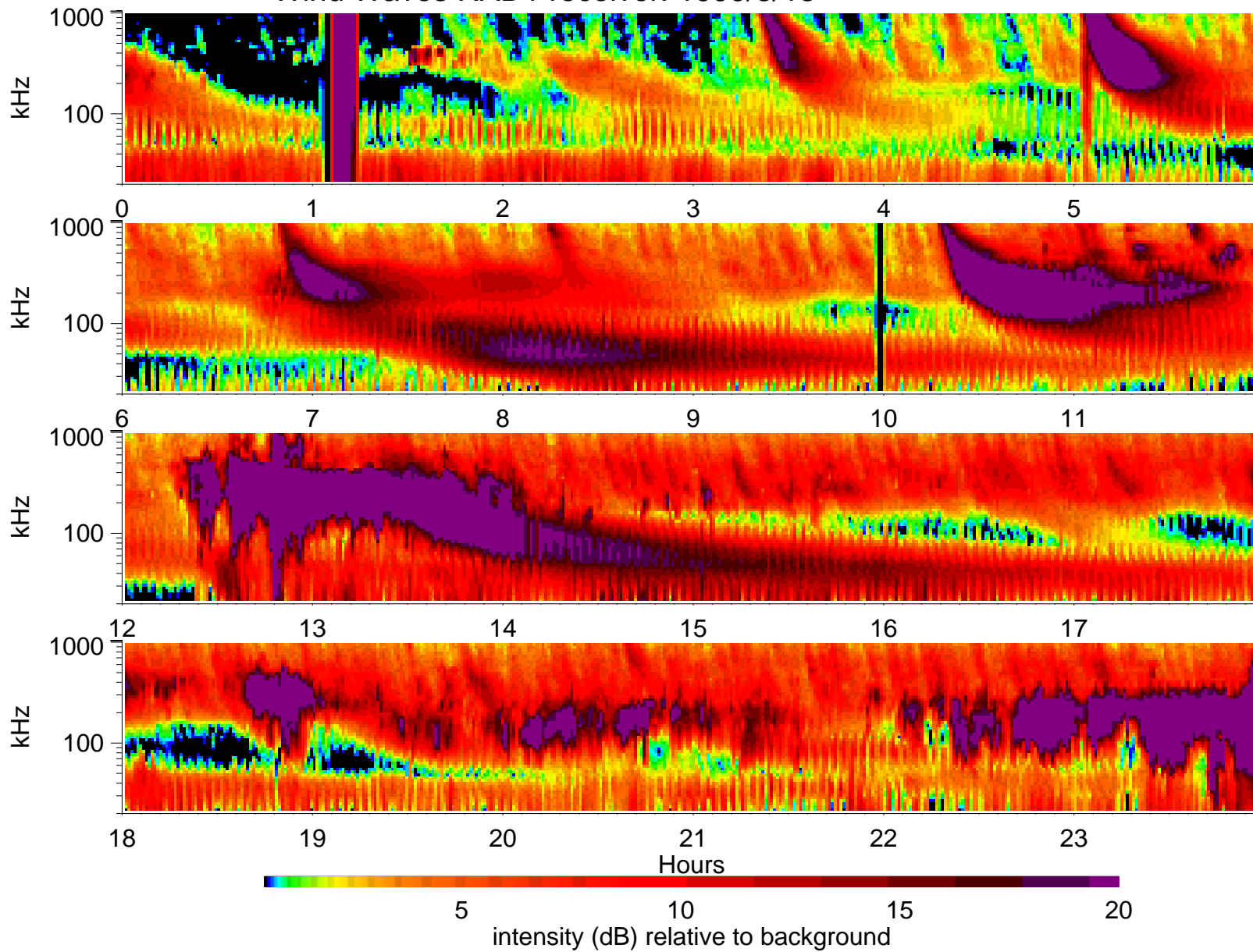
Wind Waves RAD1 receiver: 1999/3/13
