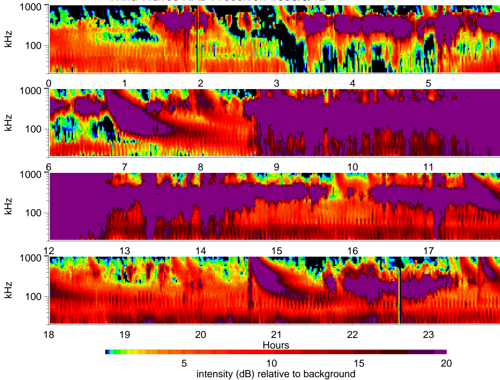
Wind Waves RAD1 receiver: 1999/3/12
