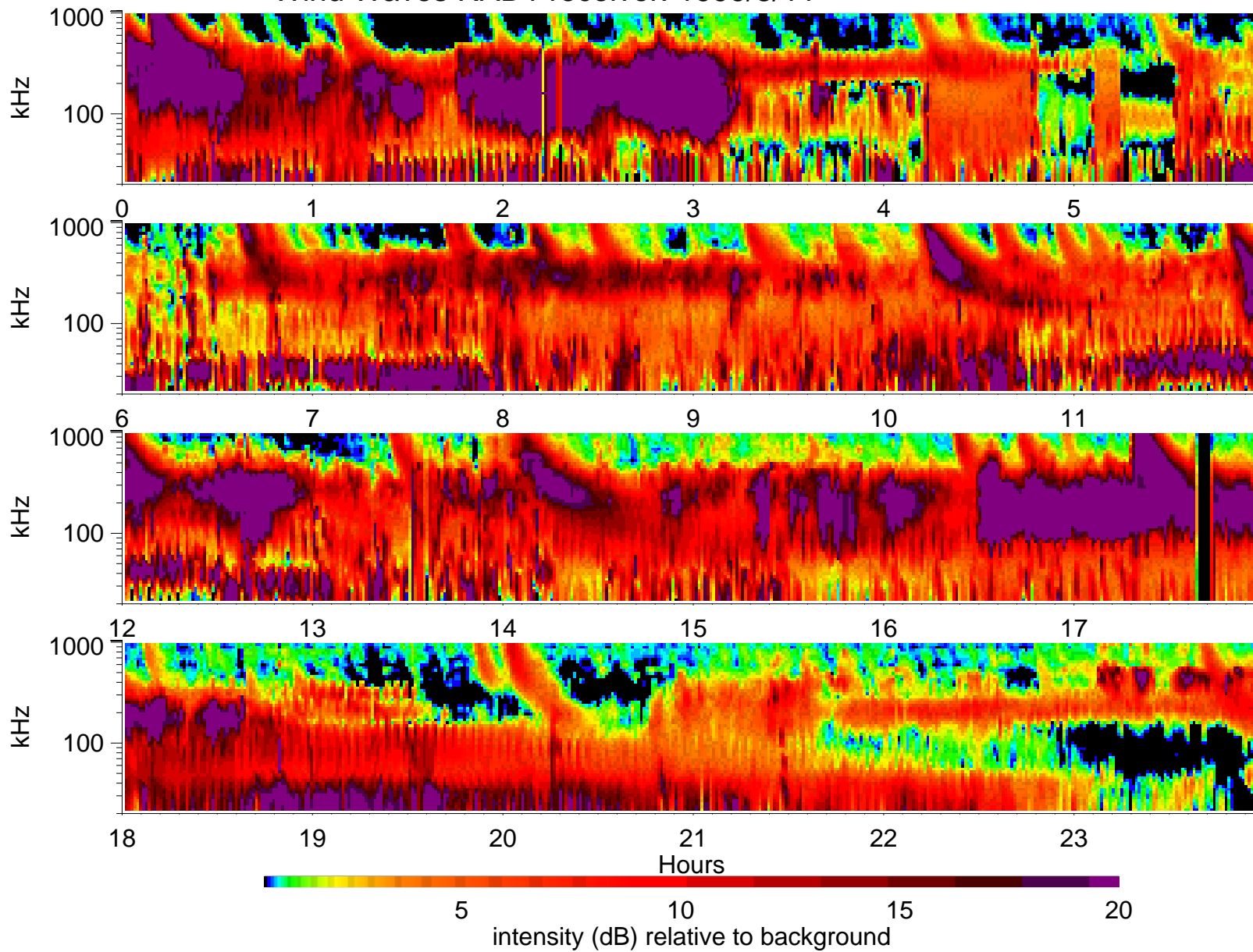
Wind Waves RAD1 receiver: 1999/3/11
