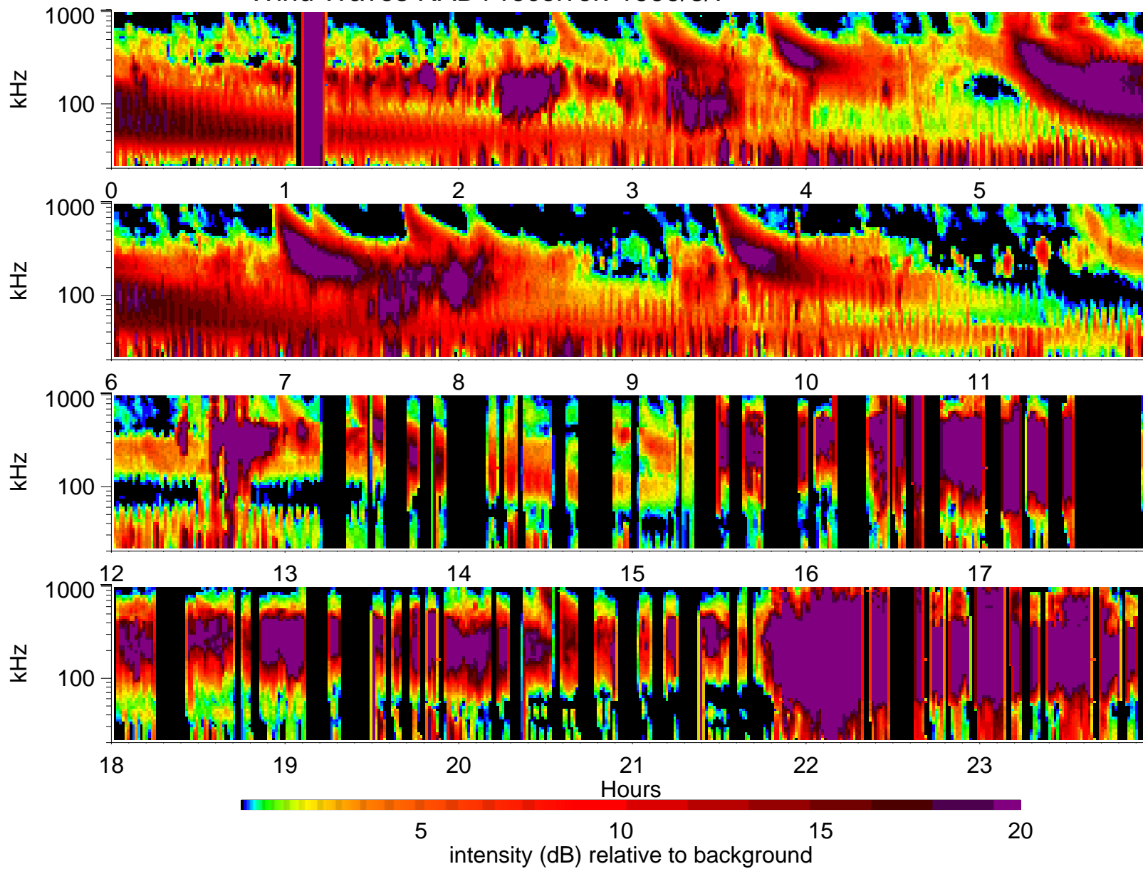
Wind Waves RAD1 receiver: 1999/3/7
