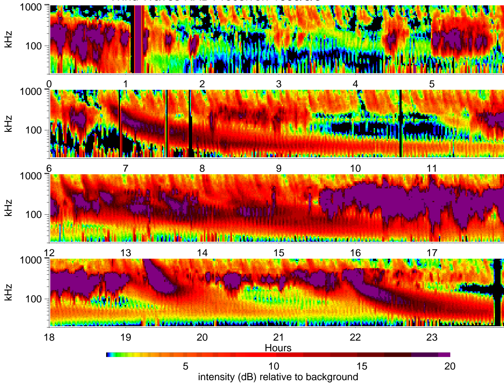
Wind Waves RAD1 receiver: 1999/3/5
