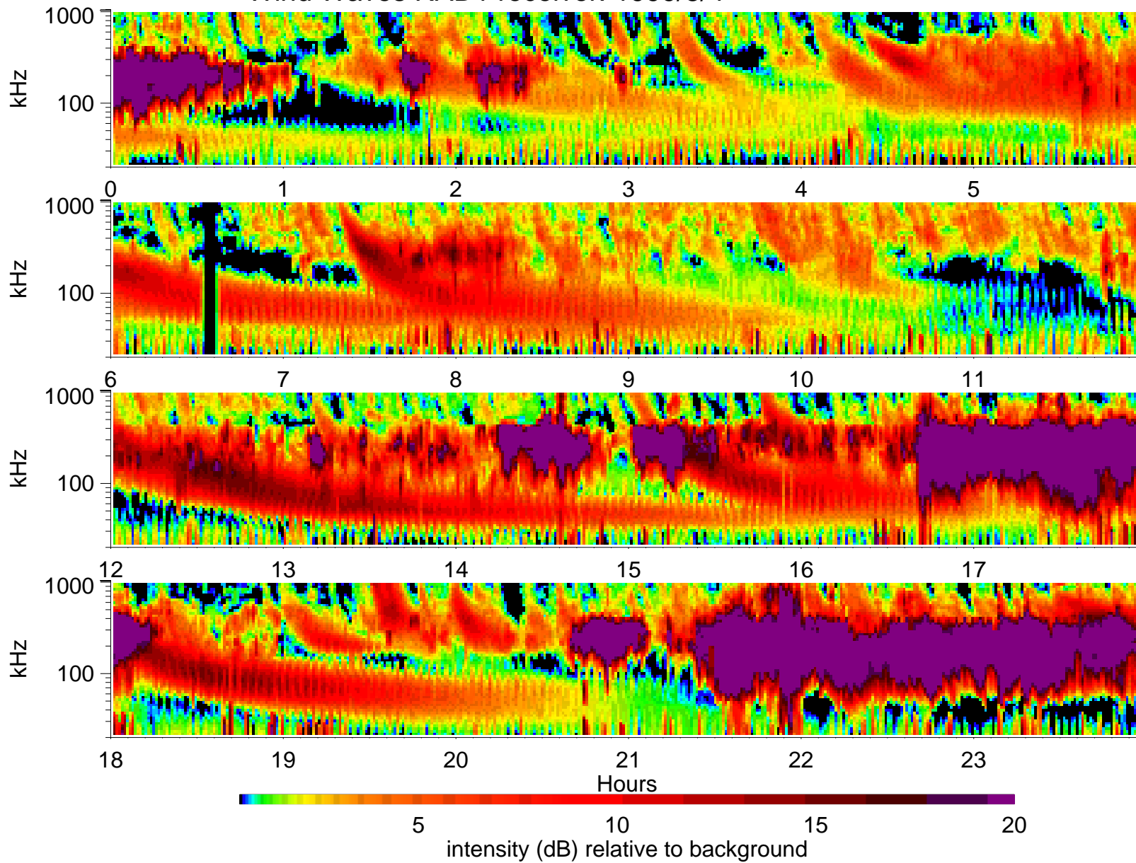
Wind Waves RAD1 receiver: 1999/3/4
