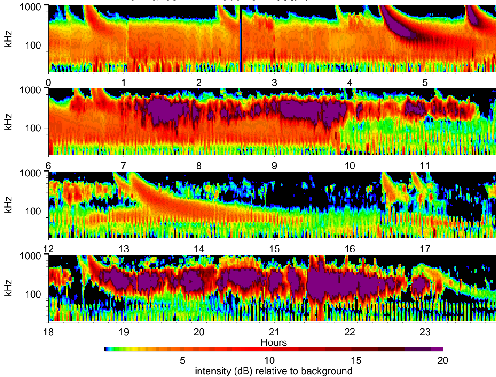
Wind Waves RAD1 receiver: 1999/2/27
