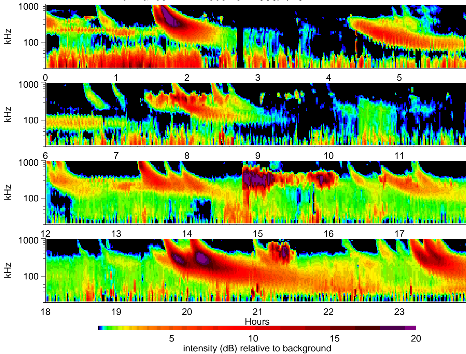
Wind Waves RAD1 receiver: 1999/2/26
