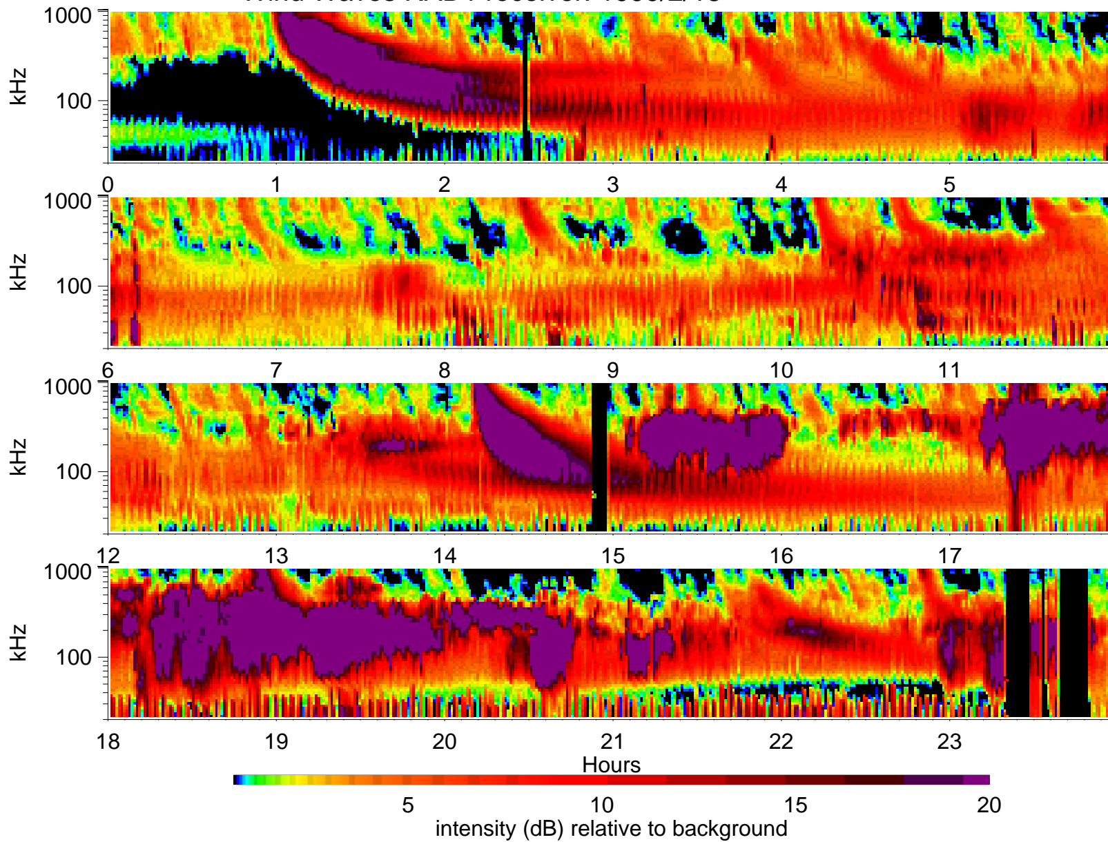
Wind Waves RAD1 receiver: 1999/2/18
