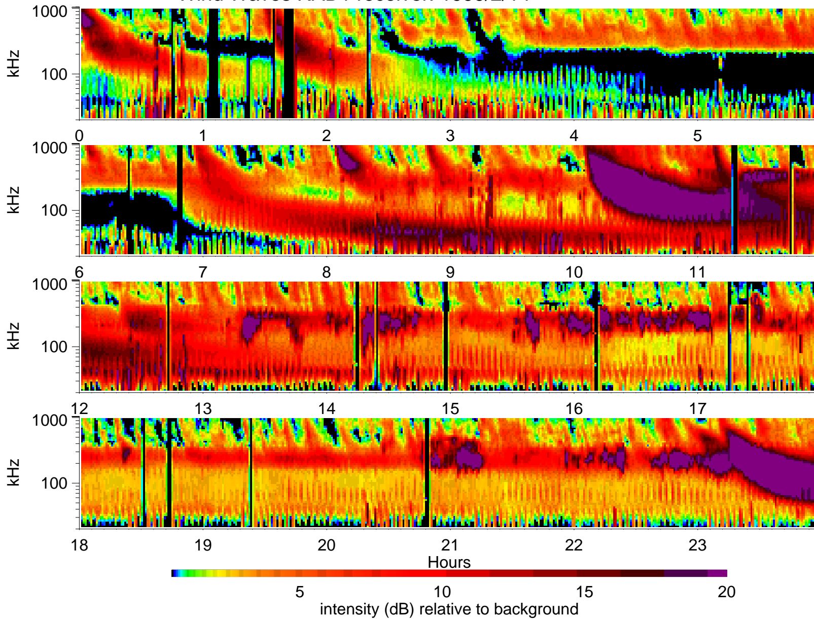
Wind Waves RAD1 receiver: 1999/2/14
