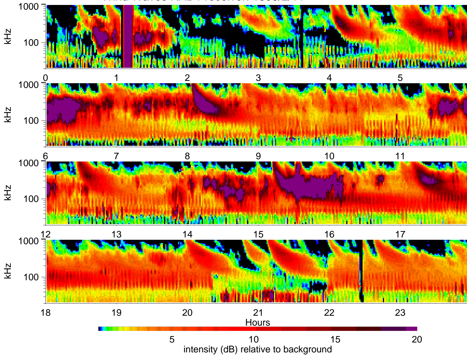
Wind Waves RAD1 receiver: 1999/2/11
