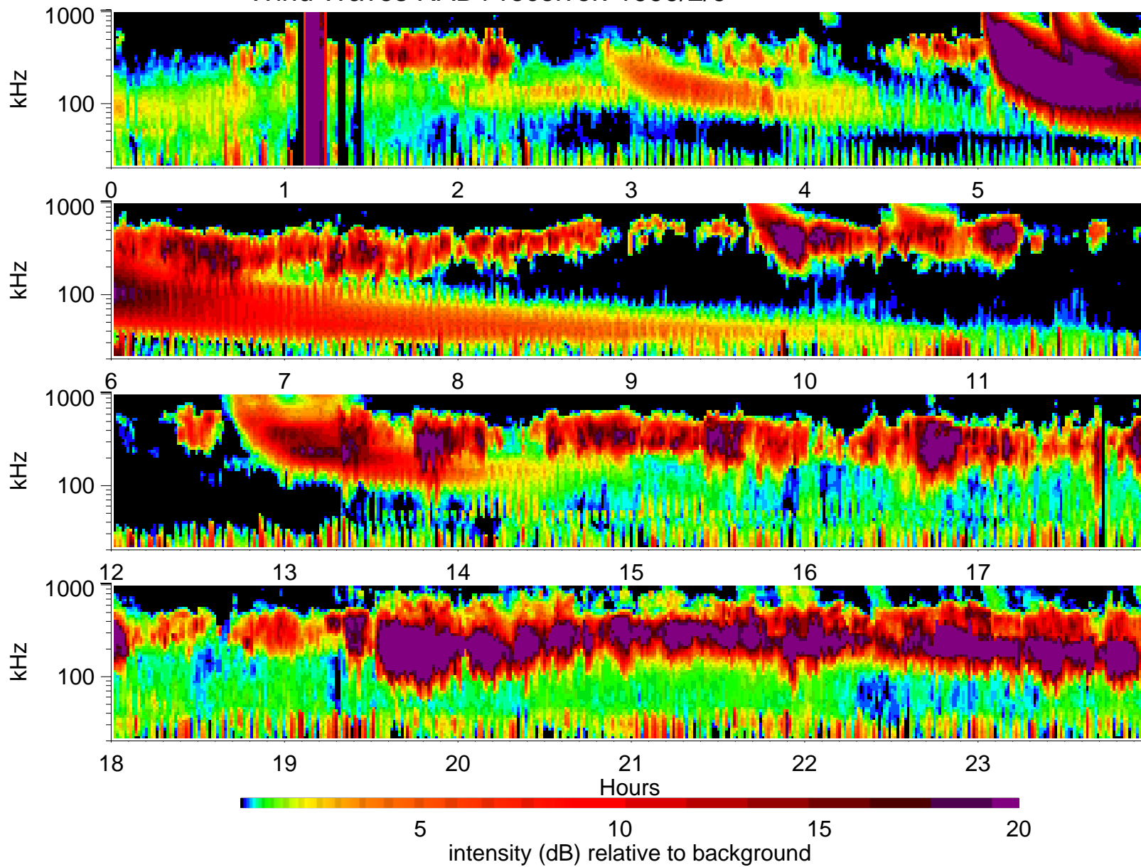
Wind Waves RAD1 receiver: 1999/2/9
