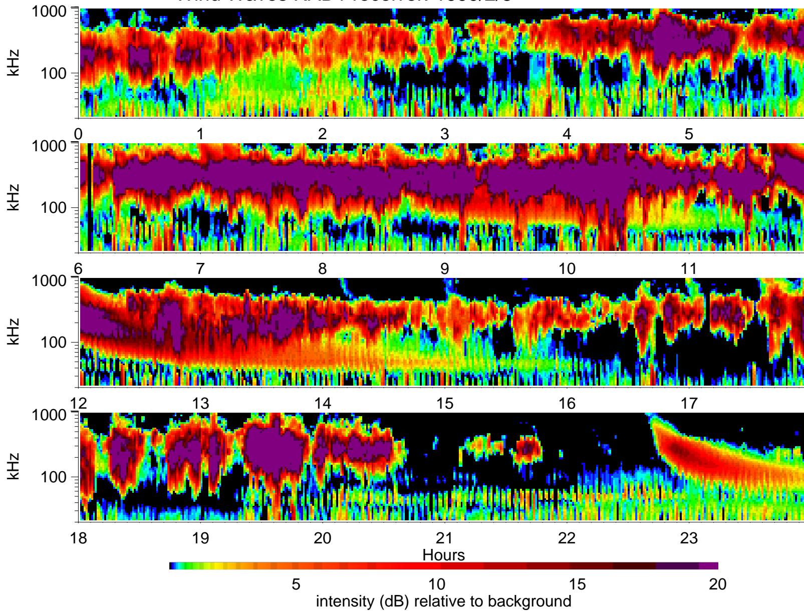
Wind Waves RAD1 receiver: 1999/2/8
