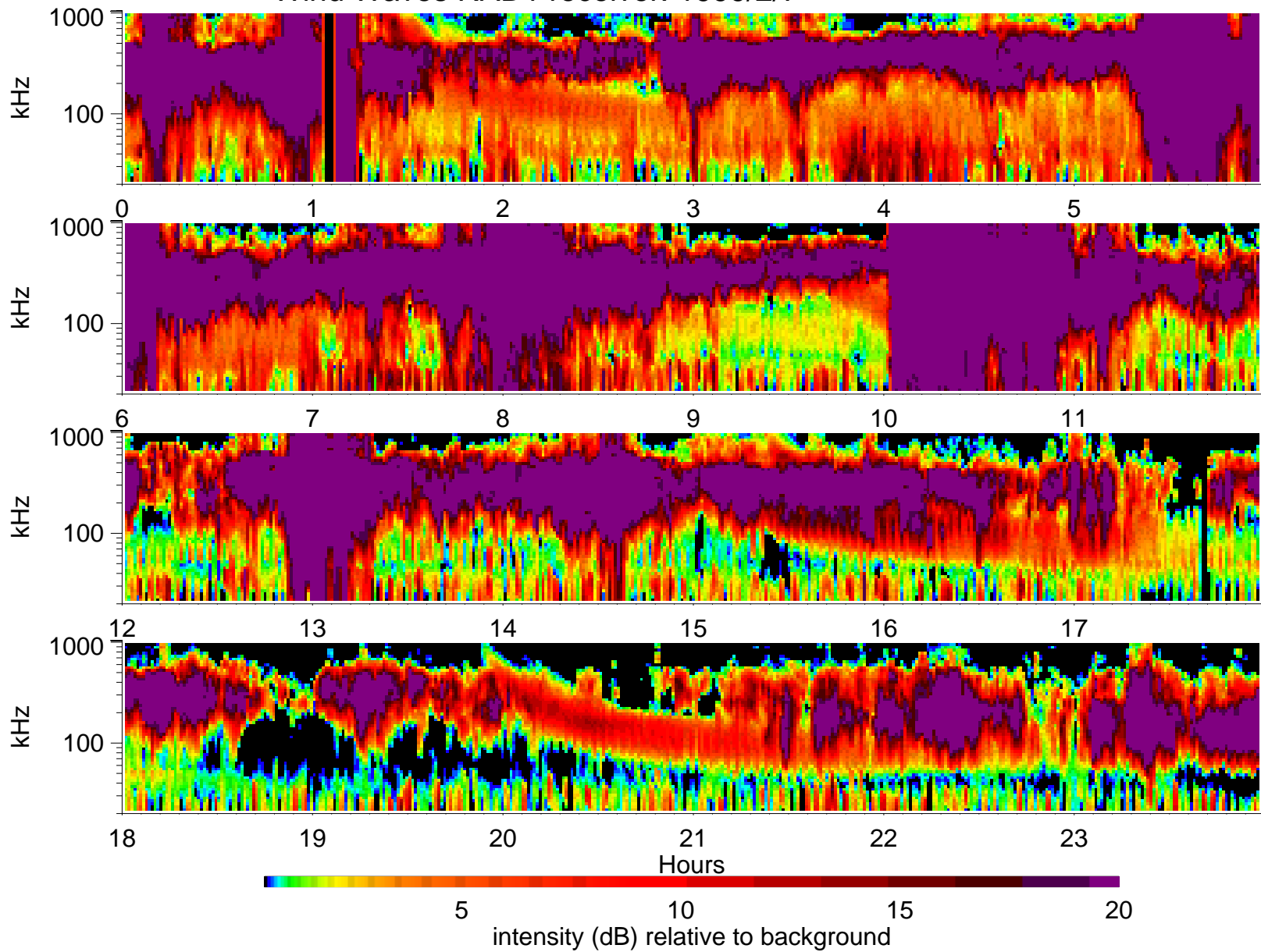
Wind Waves RAD1 receiver: 1999/2/7
