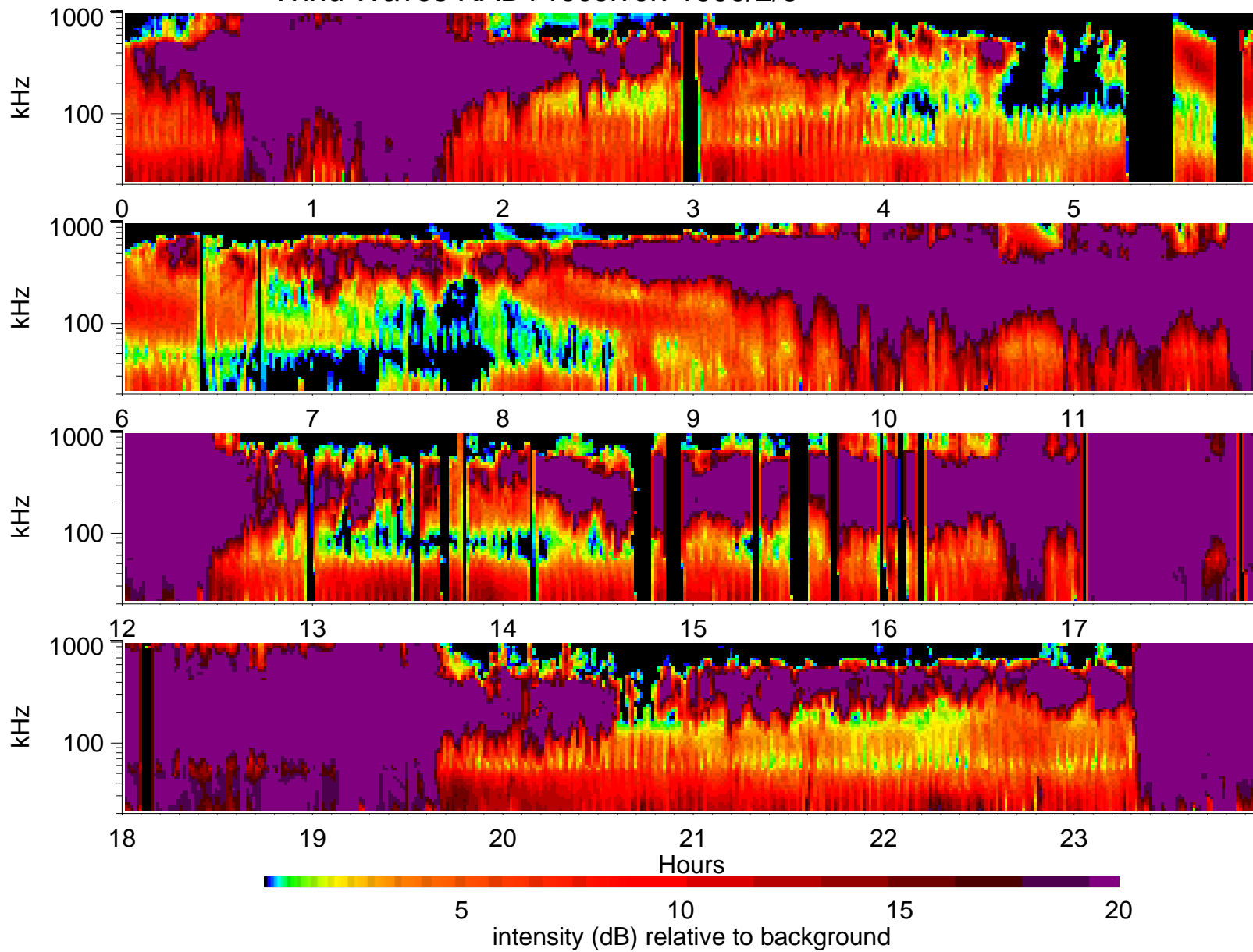
Wind Waves RAD1 receiver: 1999/2/5
