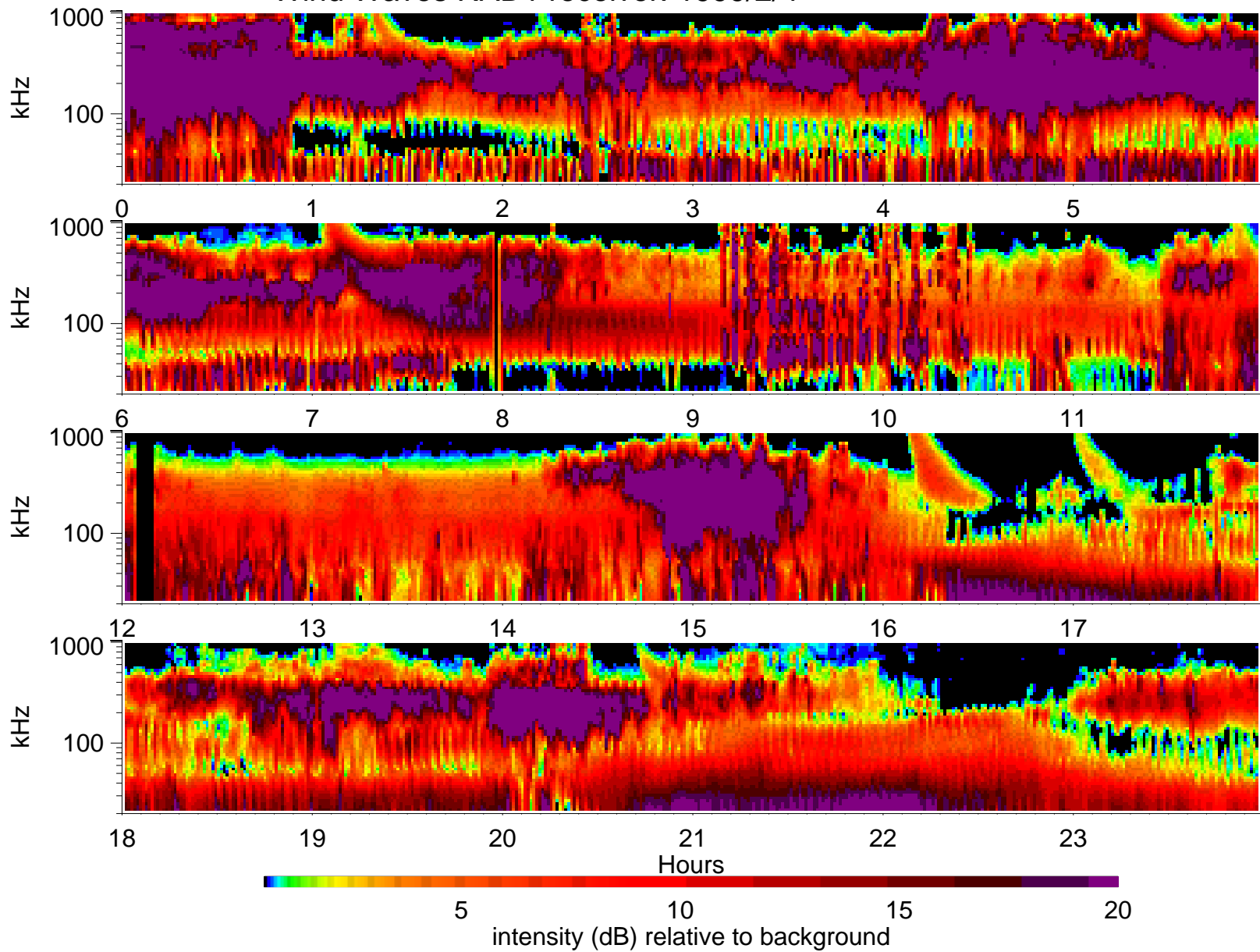
Wind Waves RAD1 receiver: 1999/2/4
