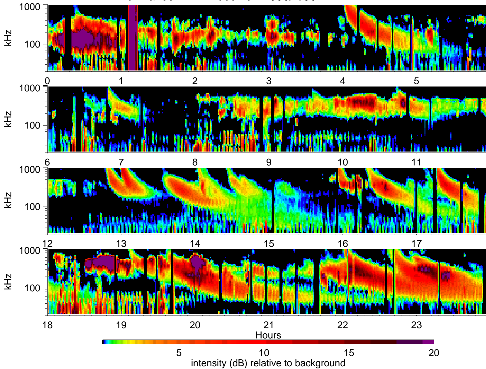
Wind Waves RAD1 receiver: 1999/1/30
