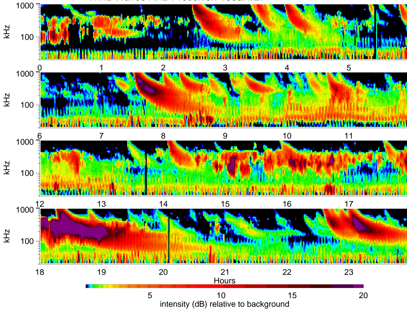
Wind Waves RAD1 receiver: 1999/1/27
